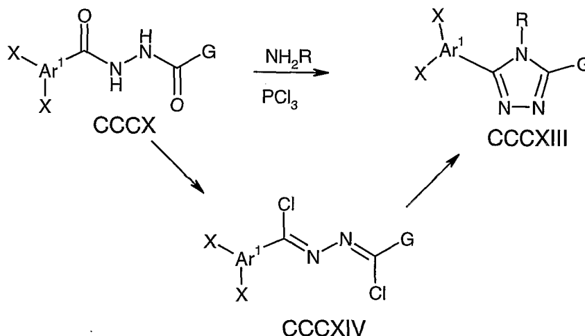
Reaction Scheme V
