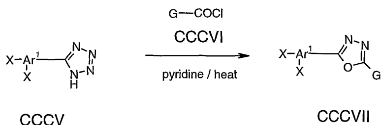
Reaction Scheme II
