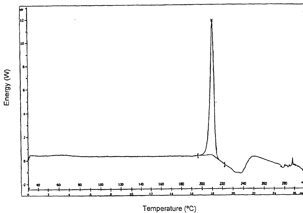
Figure 2: DSC pattern of 5-(-2-(6-(2,2-Difluoro-2-phenylethoxy) hexylamino)-1(R)-hydroxyethyl)-8-hydroxyquinolin-2(1H)-one.heminapadisylate.
