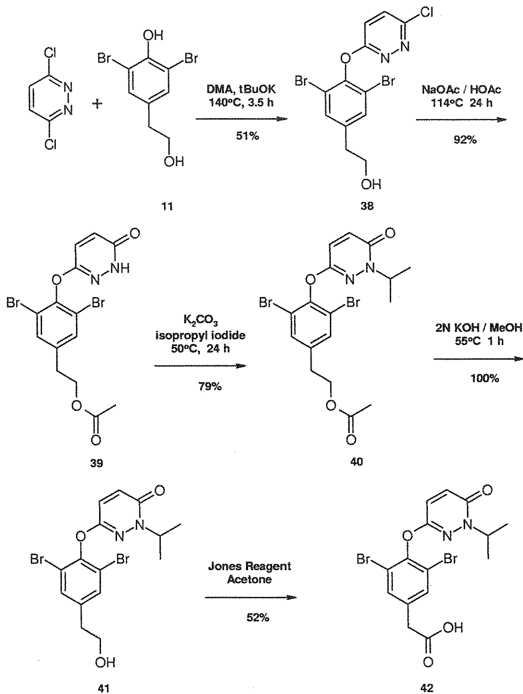
Scheme 12: Synthesis of [3,5-Dibromo-4-(1-isopropyl-6-oxo-1,6-dihydro-pyridazin-3-yloxy)-phenyl]-acetic acid (42):
