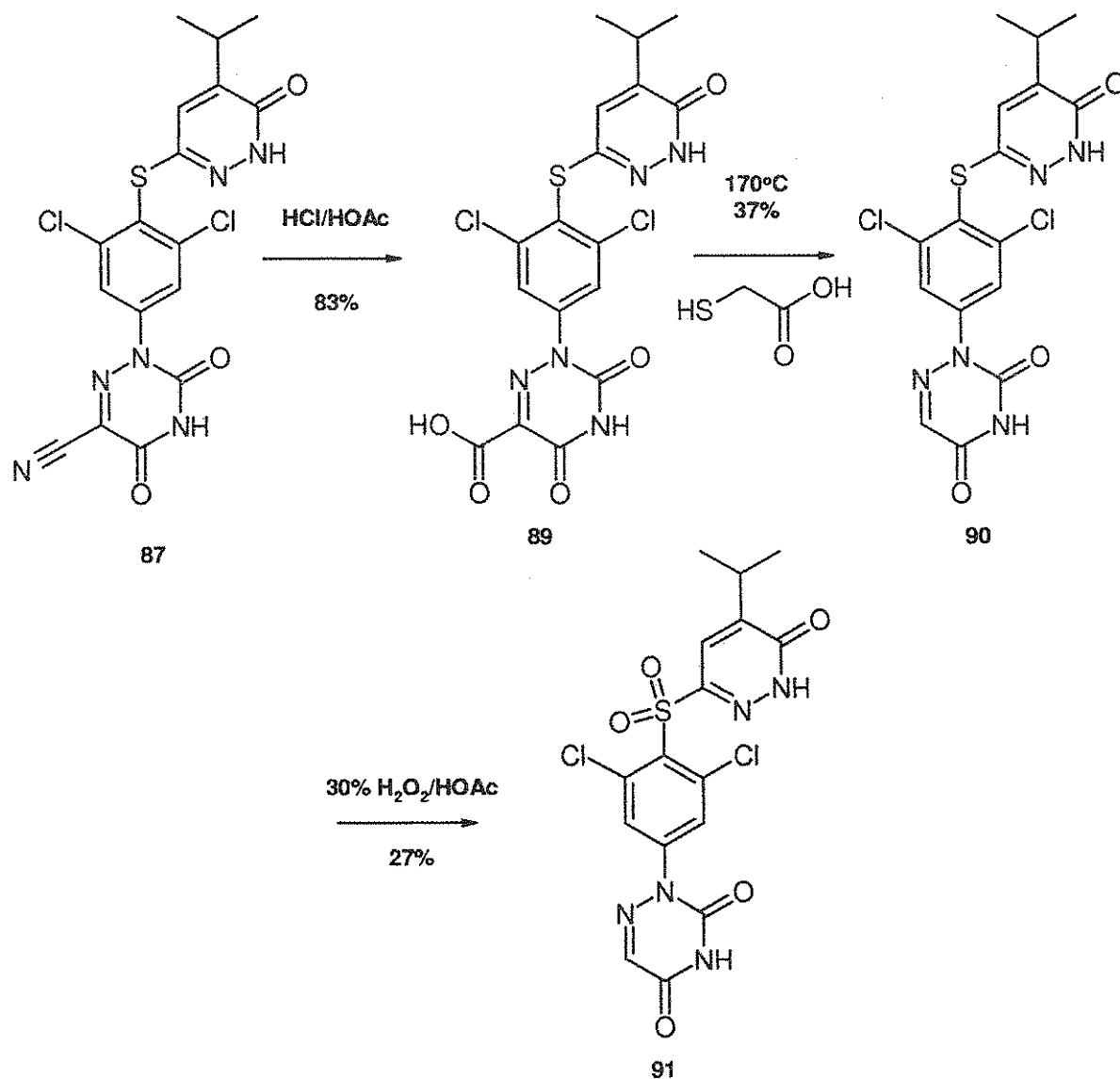
Scheme 21: Synthesis of 2-[3,5-Dichloro-4-(5-isopropyl-6-oxo-1,6-dihydro-pyridazine-3-sulfonyl)-phenyl]-2H-[1,2,4]triazine-3,5-dione (91)
