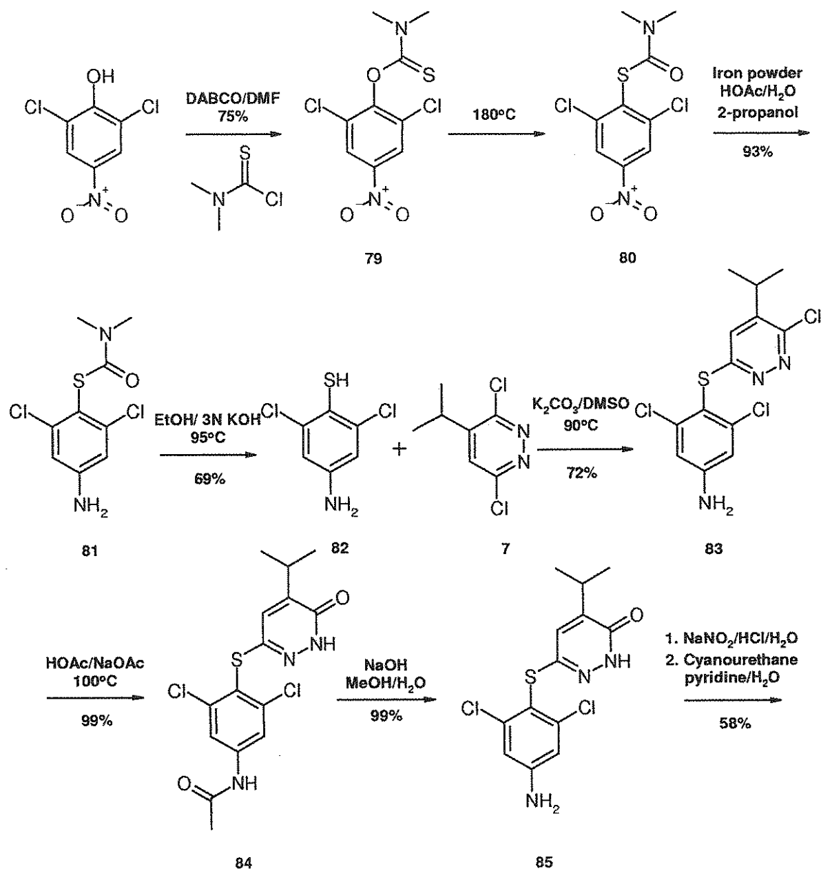
Scheme 20 : Synthesis of 2-[3,5-Dichloro-4-(5-isopropyl-6-oxo-1,6-dihydro-pyridazine-3-sulfonyl)-phenyl]-3,5-dioxo-2,3,4,5-tetrahydro-[1,2,4]triazine-6-carbonitrile (88)
