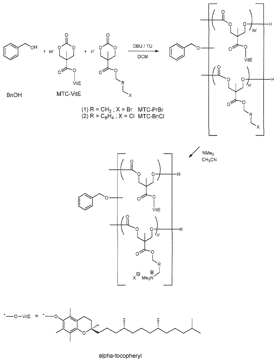
Scheme 1.
