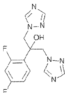
(Fluconazole)
