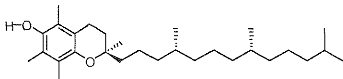
(alpha-tocopherol),
