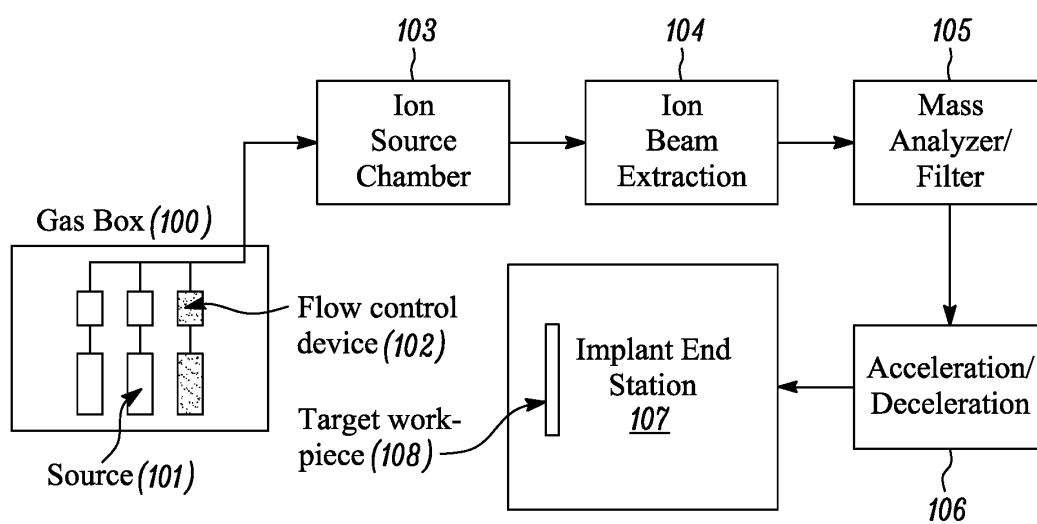
Schematic of beamline ion implant system
