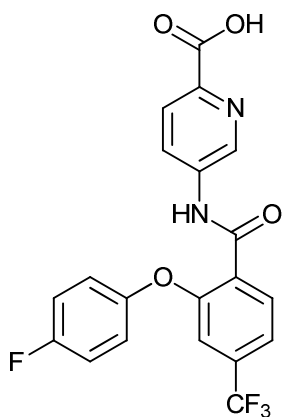
5-(2-(4-fluorophenoxy)-4-(trifluoromethyl)benzamido)picolinic acid;
