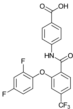
4-(2-(2,4-difluorophenoxy)-4-(trifluoromethyl)benzamido)benzoic acid;
