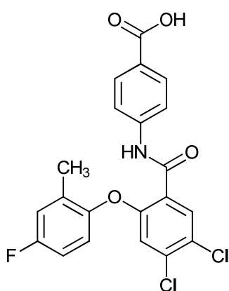
4-(4,5-dichloro-2-(4-fluoro-2-methylphenoxy)benzamido)benzoic acid;
