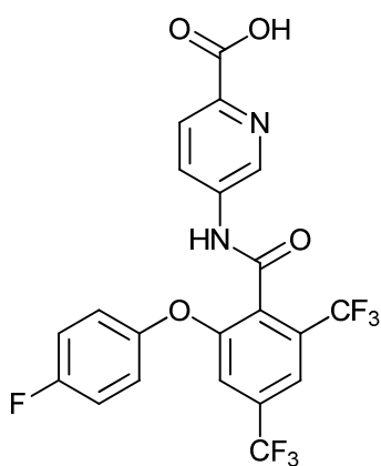
5-(2-(4-fluorophenoxy)-4,6-bis(trifluoromethyl)benzamido)picolinic acid;
