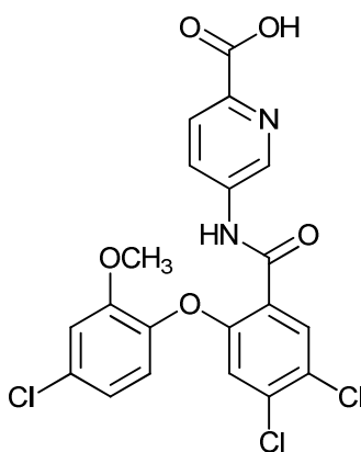
5-(4,5-dichloro-2-(4-chloro-2-methoxyphenoxy)benzamido)picolinic acid;
