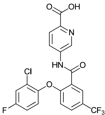
5-(2-(2-chloro-4-fluorophenoxy)-5-(trifluoromethyl)benzamido)picolinic acid;
