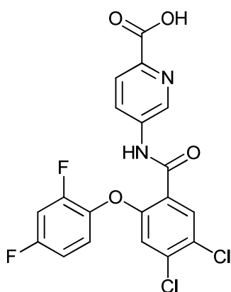
5-(4,5-dichloro-2-(2,4-difluorophenoxy)benzamido)picolinic acid;
