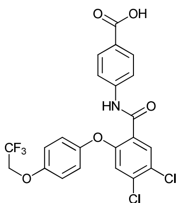
4-(4,5-dichloro-2-(4-(2,2,2-trifluoroethoxy)phenoxy)benzamido)benzoic acid;
