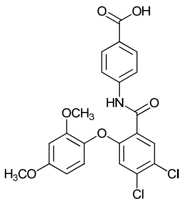
4-(4,5-dichloro-2-(2,4-dimethoxyphenoxy)benzamido)benzoic acid;
