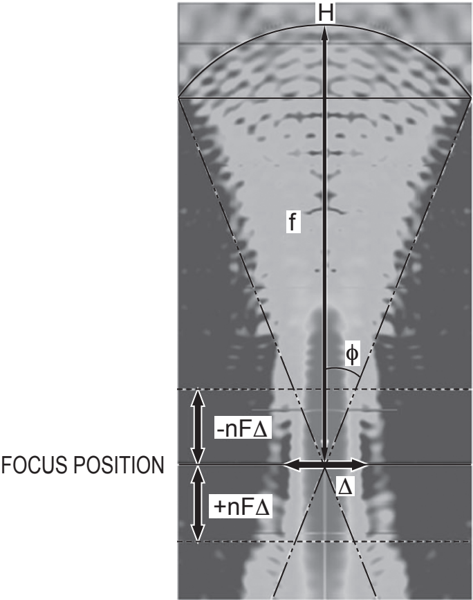
SECTIONAL VIEW PARALLEL TO OPTICAL AXIS
