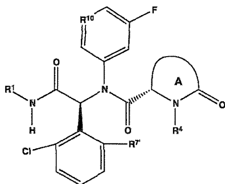
formula II-b
