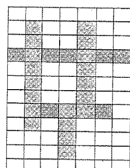
Liquidus detected
