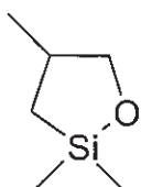
2,2,4-trimethyl-1-oxa-2-silacyclopentane
