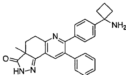
7-(4-(1-aminocyclobutyl)phenyl)-3a-methyl-8-phenyl-4,5-dihydro-2H-pyrazolo[3,4-f]quinolin-3(3aH)-one
