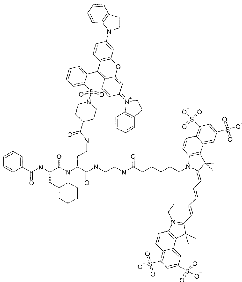
(Scheme 4)
