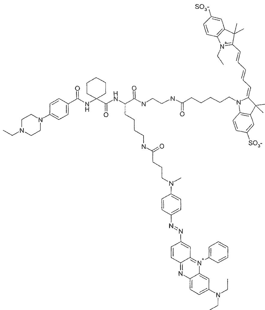
(Scheme 9)
