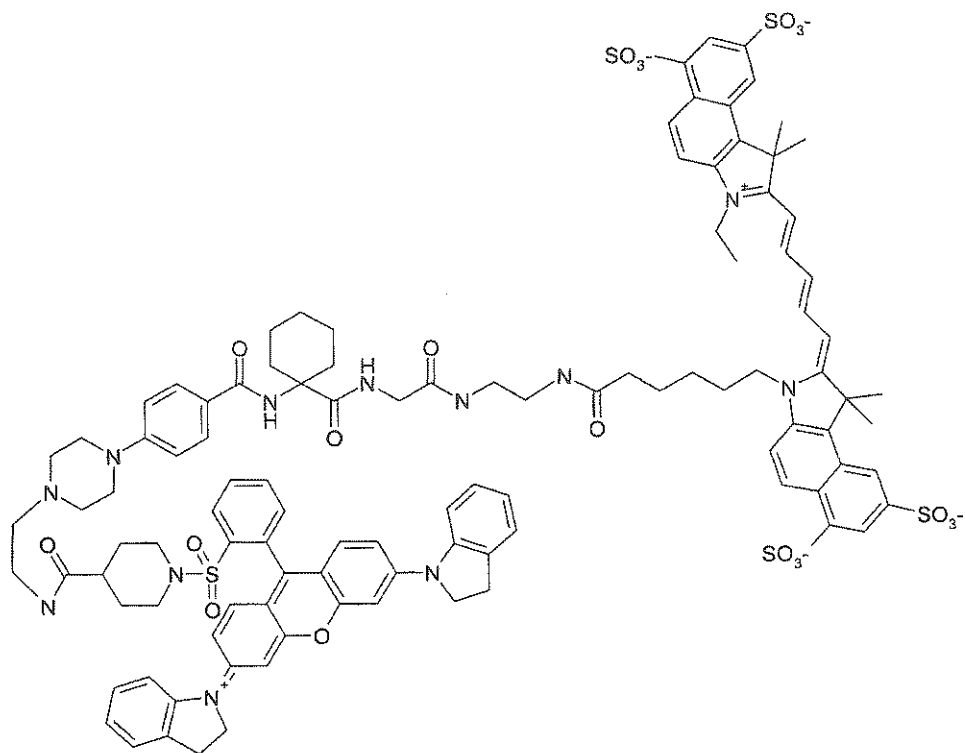
(Scheme 10)
