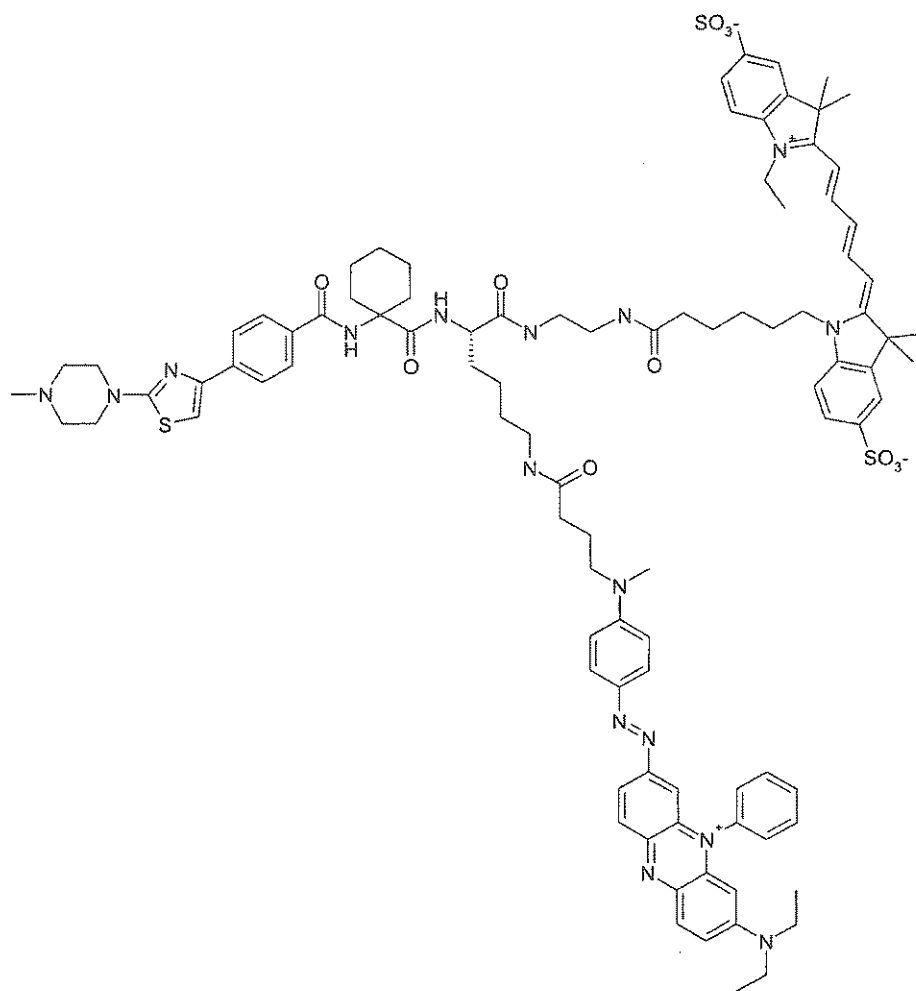
(Scheme 13)
