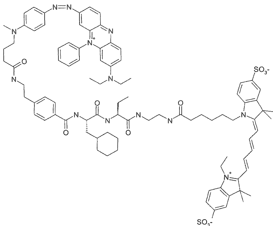
(Scheme 7)
