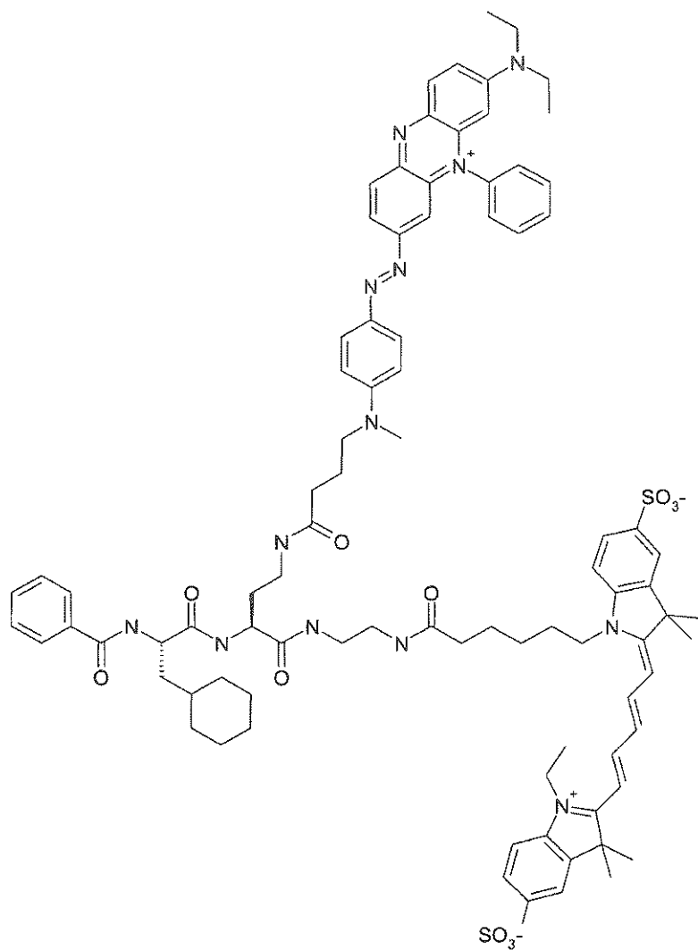
(Scheme 6)
