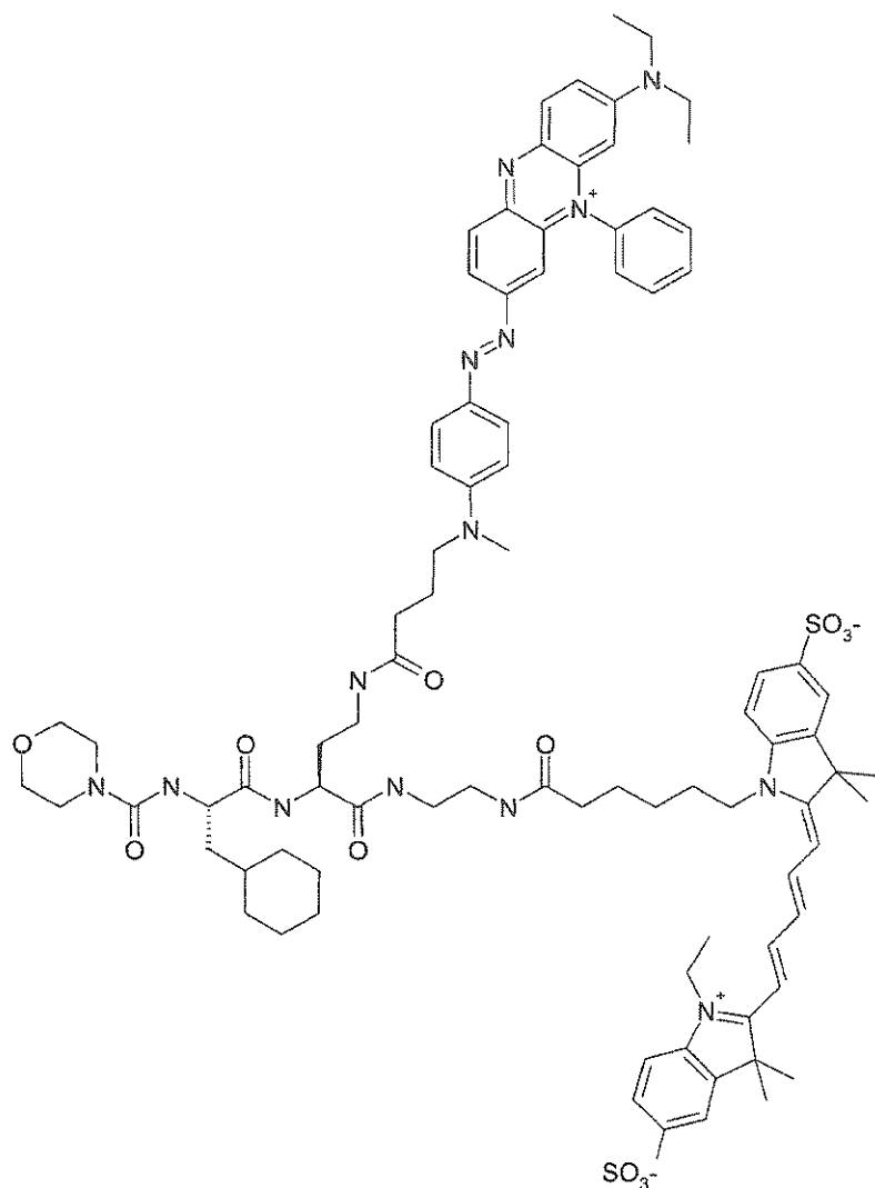
(Scheme 3)
