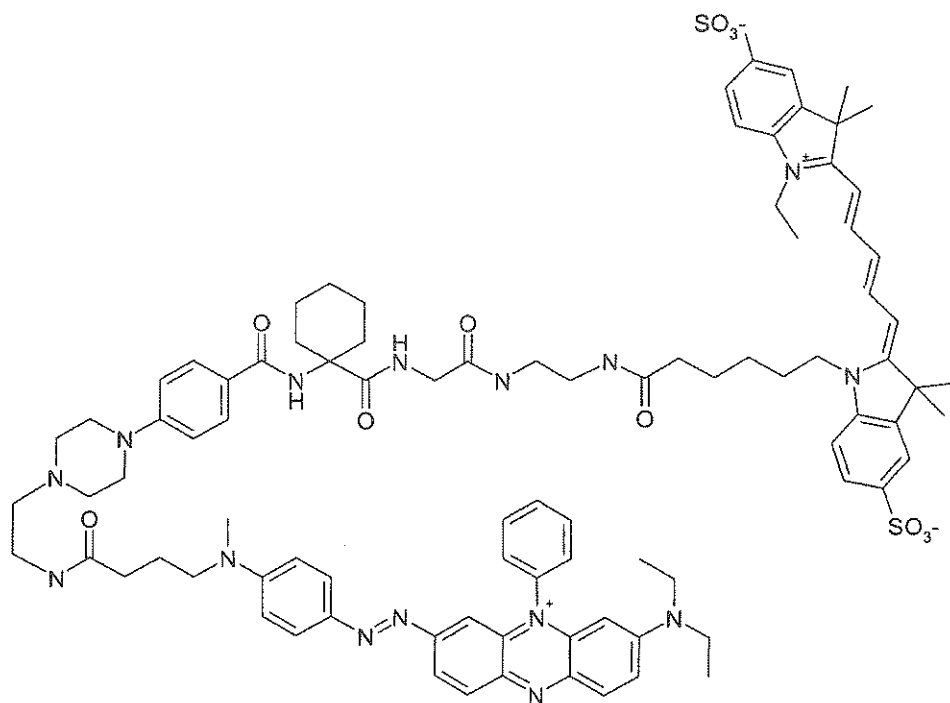
(Scheme 11)
