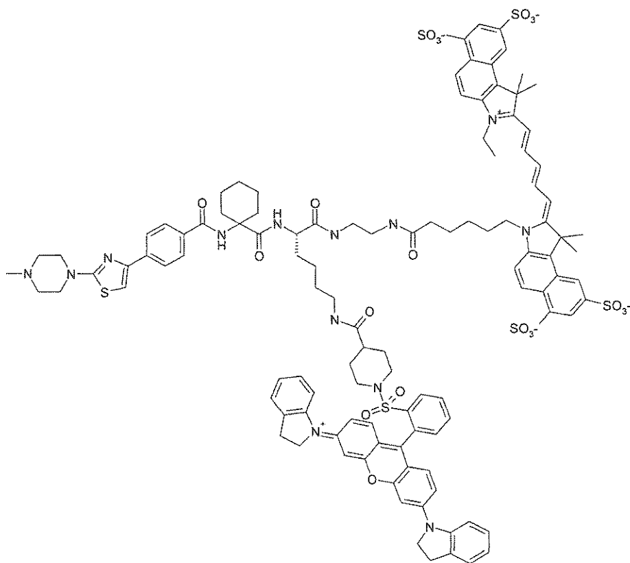
(Scheme 12)
