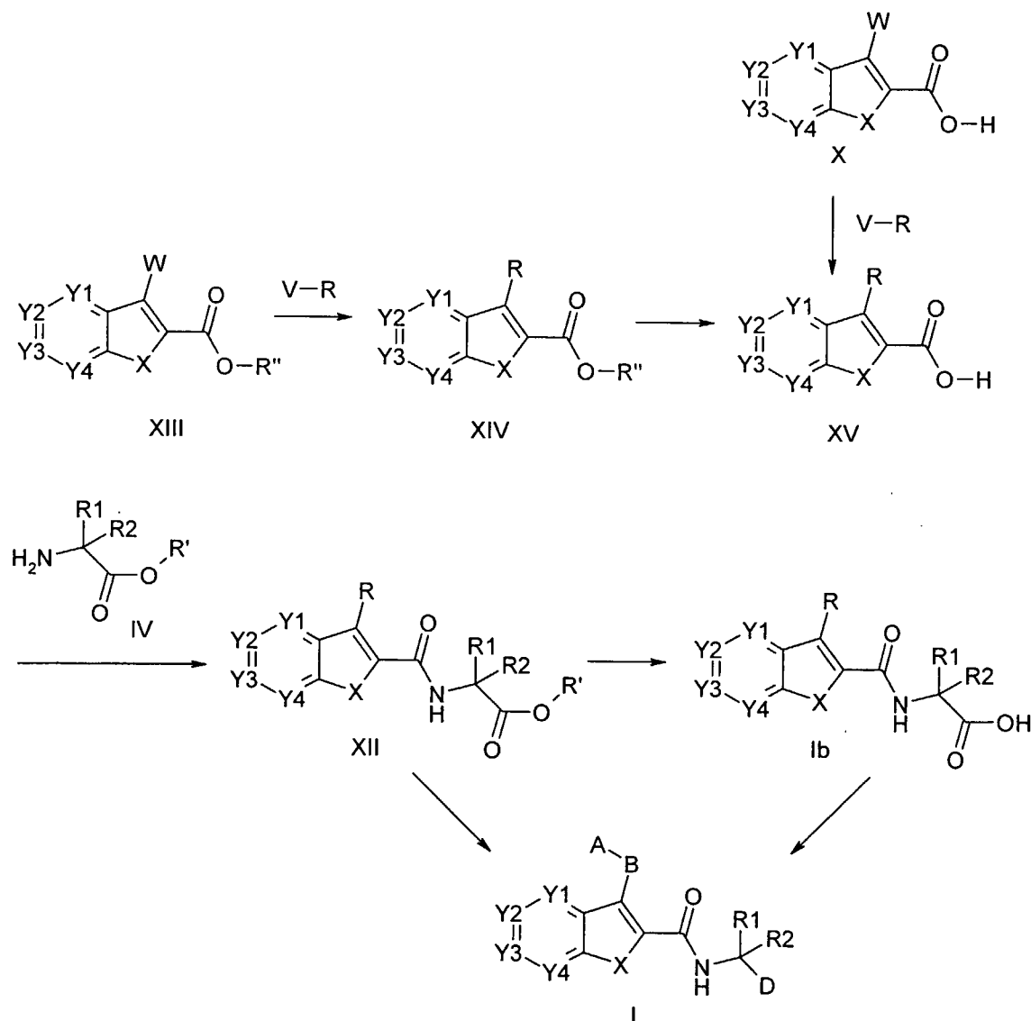
Scheme 4
