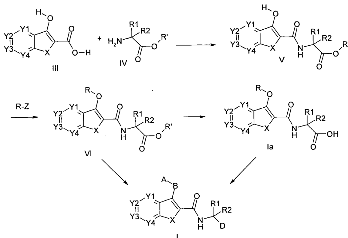
Scheme 1
