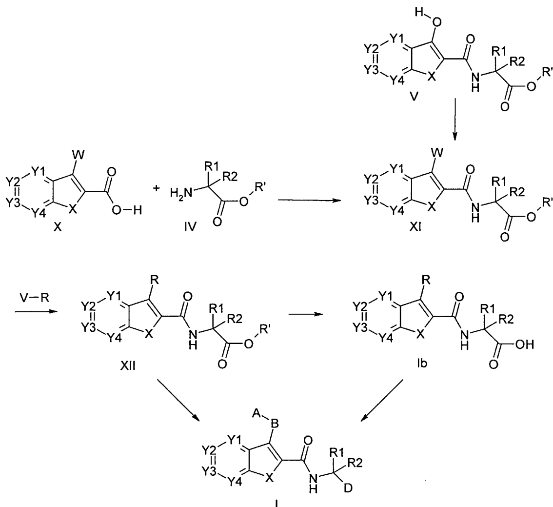
Scheme 3
