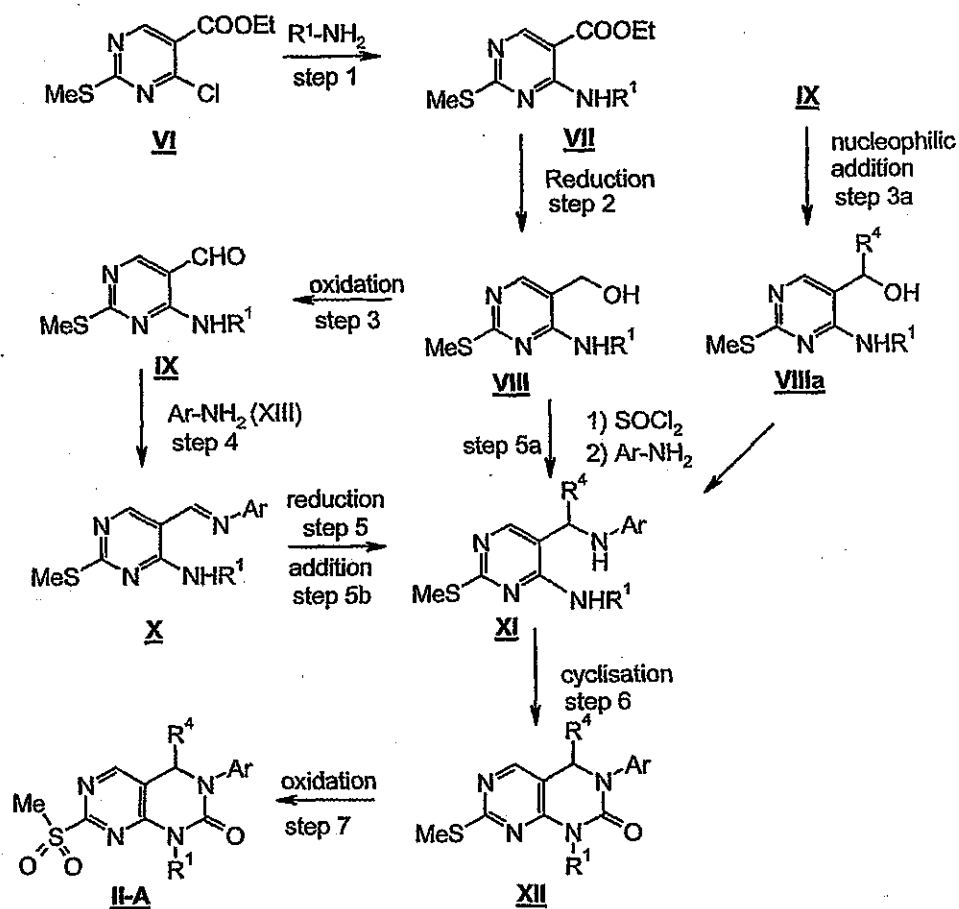
Scheme 2
