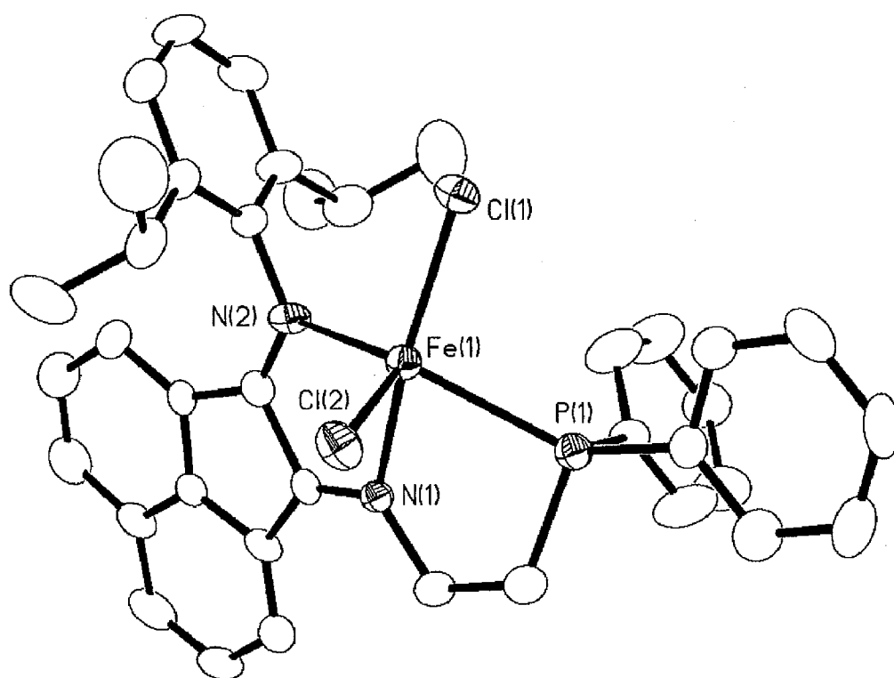
Figure 1 – ORTEP Diagram of the X-Ray Crystal Structure for the \alpha -Diimine Metal Complex Produced in Example 5
