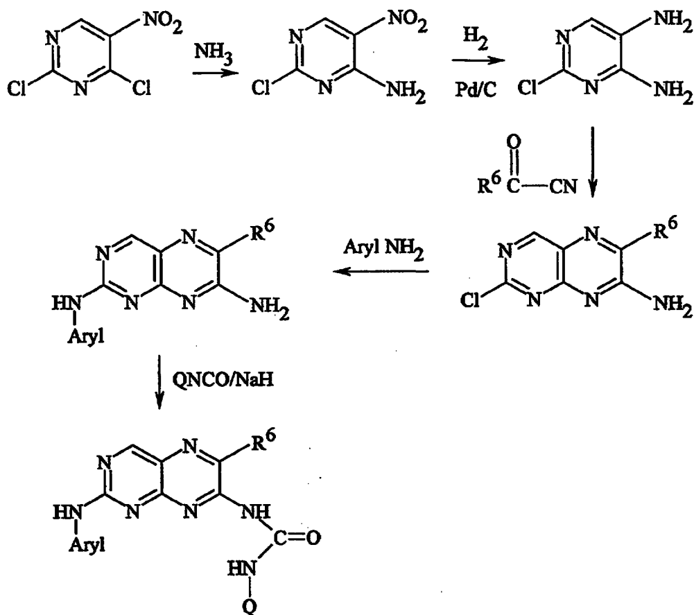
Scheme IV
