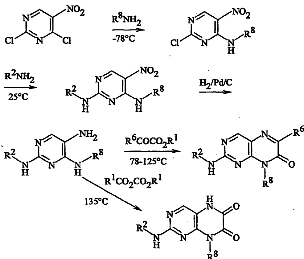
Scheme I
