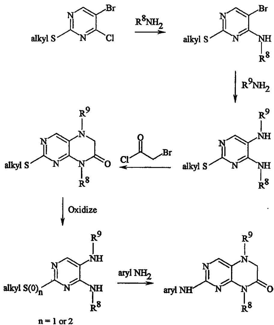
Scheme III
