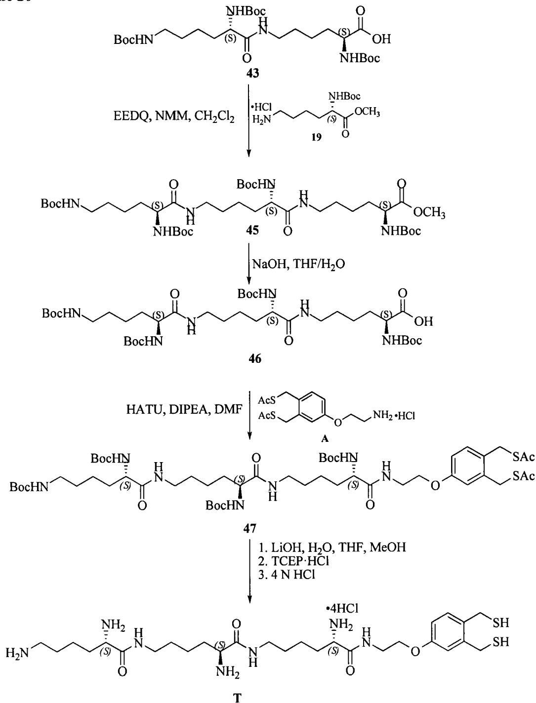
Scheme 20
