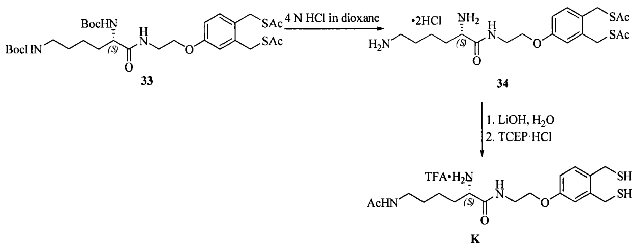
Scheme 11
