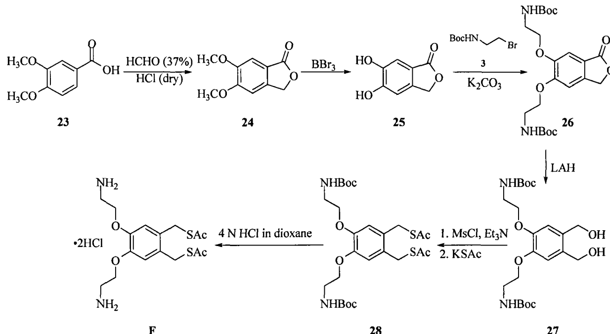
Scheme 6
