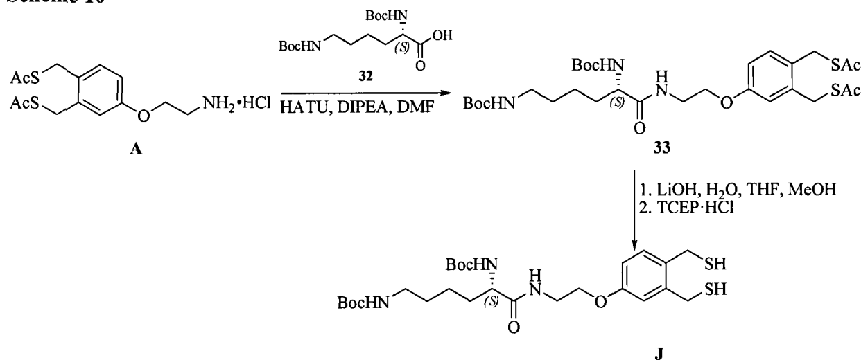
Scheme 10
