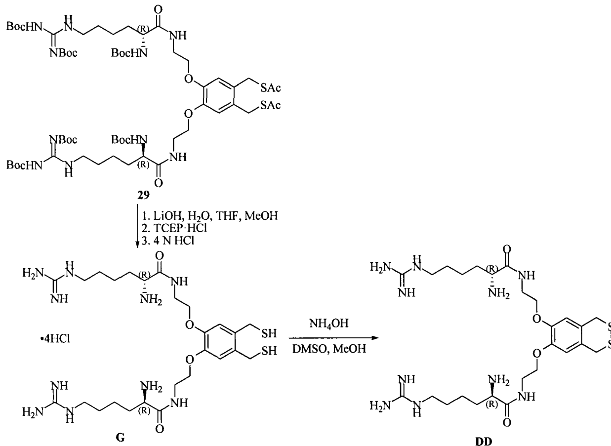
Scheme 30
