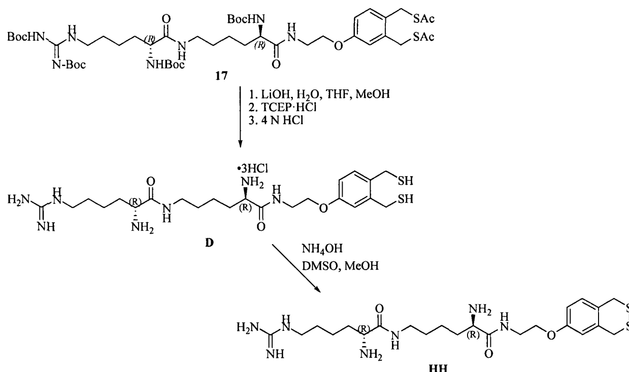
Scheme 34
