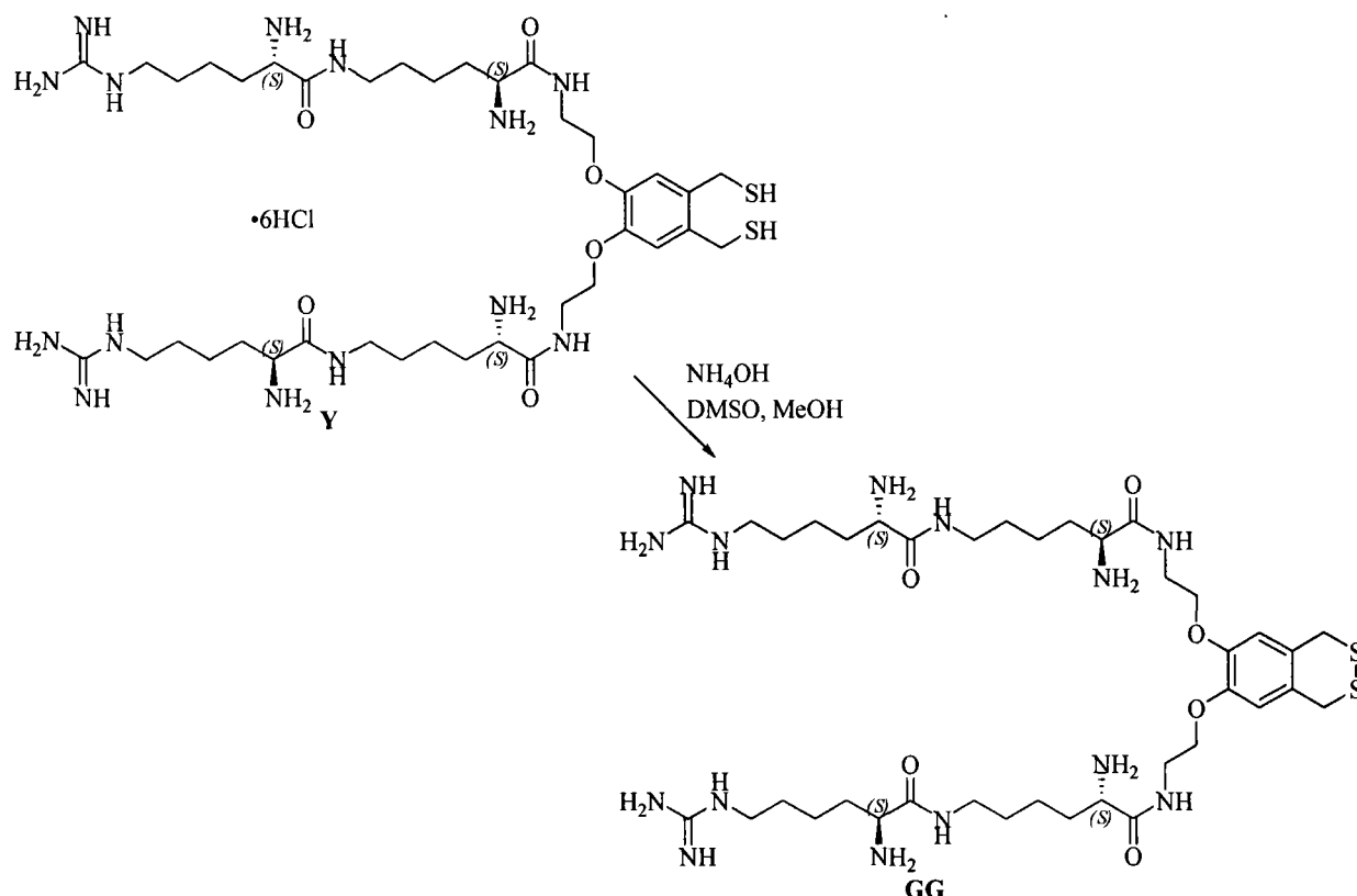
Scheme 33
