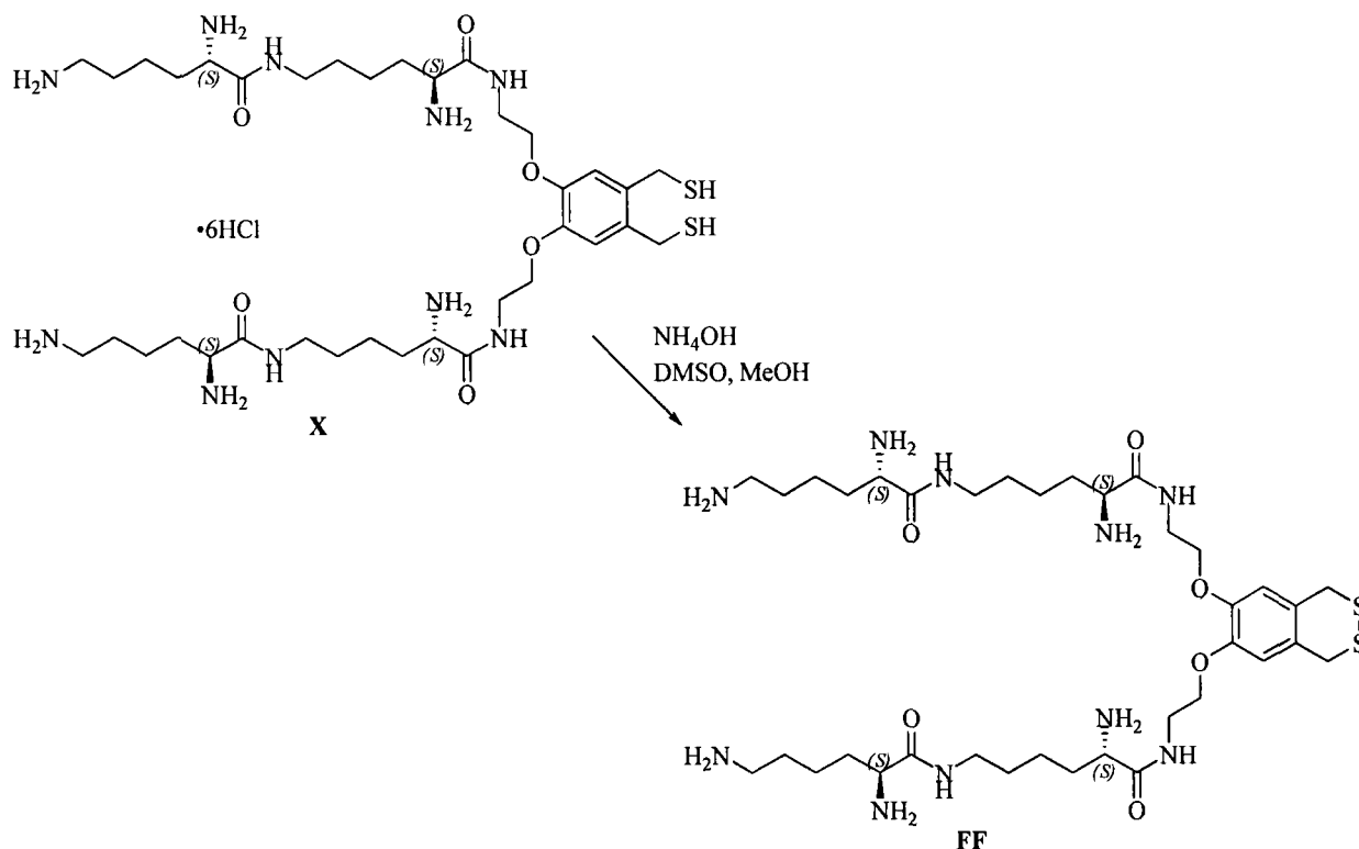
Scheme 32
