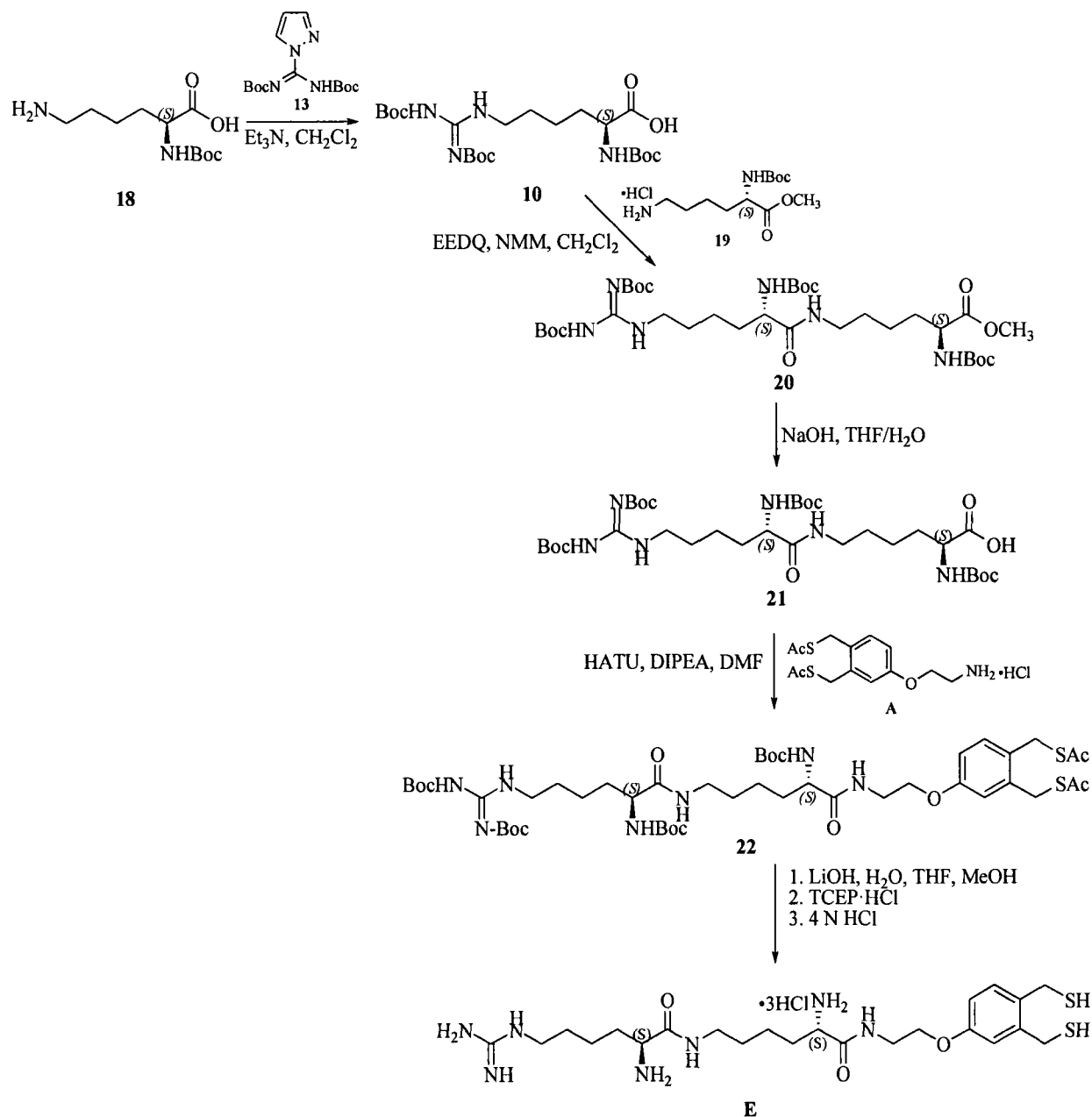
Scheme 5
