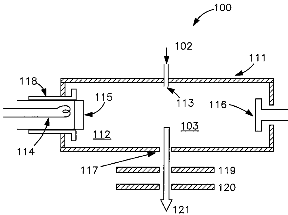
Schematic of an ion source apparatus
