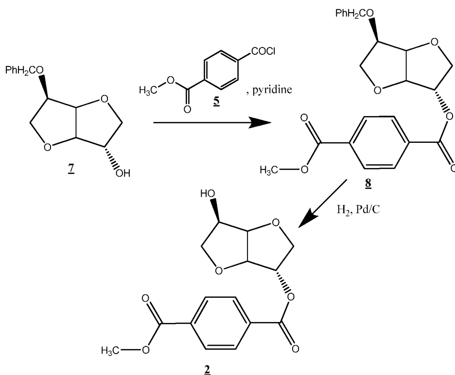
Scheme 2: Isosorbide 2-(4-carbomethoxybenzoate), Isosorbide 2-TA AB monomer ( 2 )
