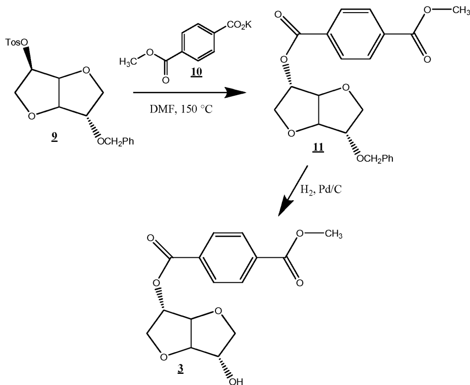
Scheme 3: Isoidide 2-(4-carbomethoxybenzoate), Isoidide 2-TA AB monomer
