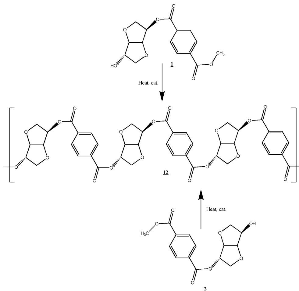
Scheme 5: Synthesis of stereoregular PEIT (12) from AB monomers 1 or 2.
