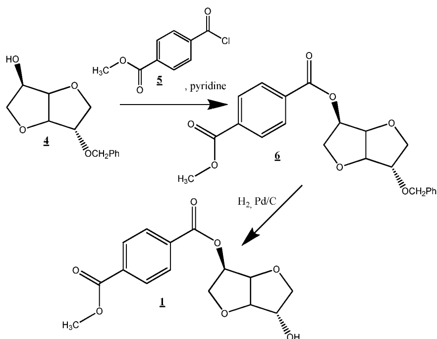
Scheme 1: Isosorbide 5-(4-carbomethoxybenzoate), Isosorbide 5-TA AB monomer 1
