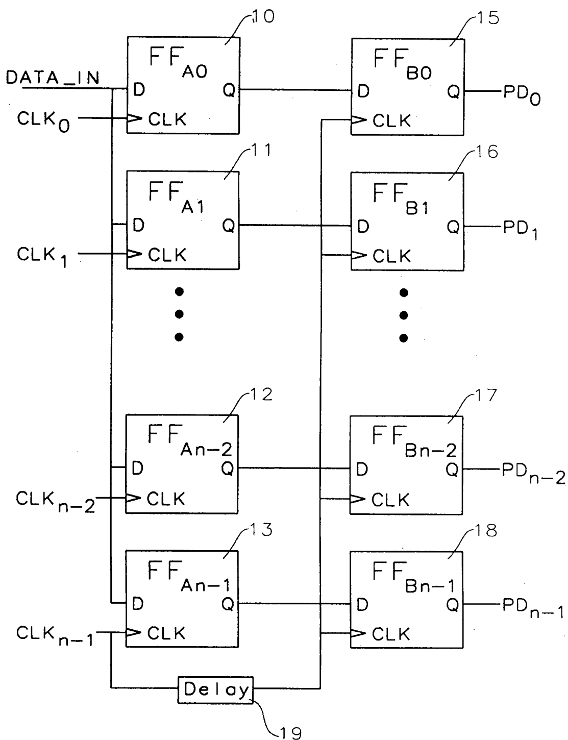
FIG. 1 Prior Art
