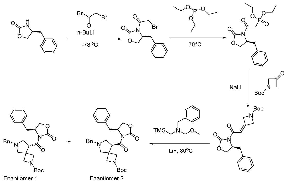
Scheme 3: Synthesis of Individual Enantiomers via Separation of Intermediates using Oxazolidinone Auxiliary
