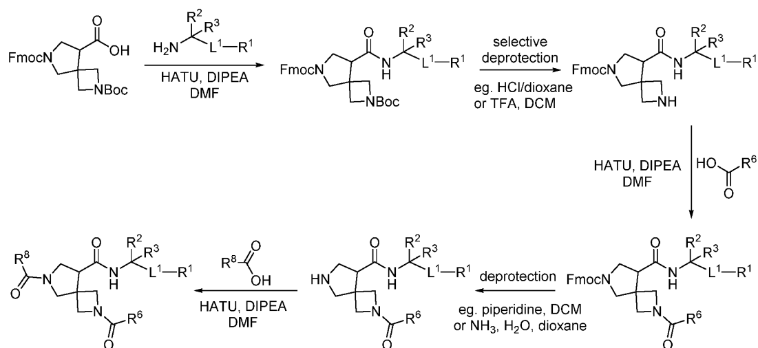
Scheme 2: Racemic Functionalization of Spirocyclic Core Structure
