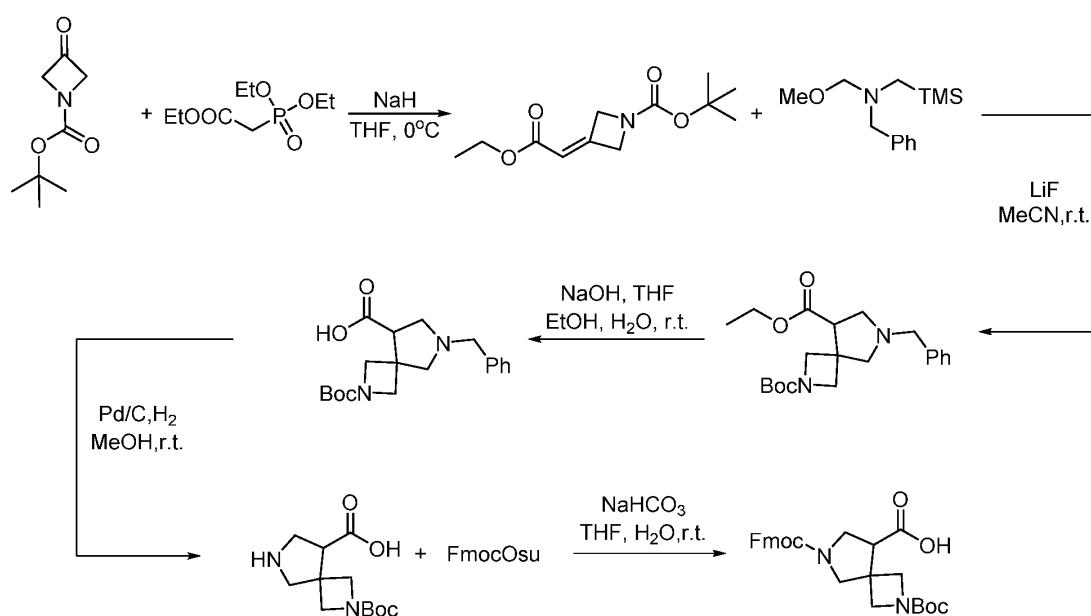
Scheme 1: Synthesis of Spirocyclic Core Structure
