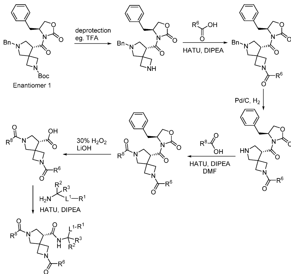
Scheme 4: Synthesis of Individual Enantiomers from Separated Intermediates
