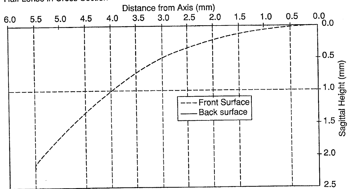
Half Lense in Cross Section
