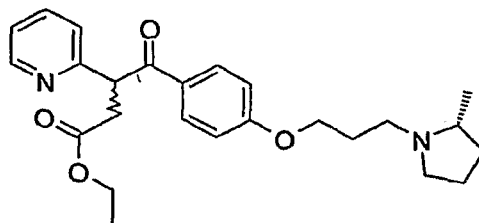
4-{4-[3-((R)-2-Methyl-pyrrolidin-1-yl)-propoxy]-phenyl}-4-oxo-3-pyridin-2-yl-butanoic acid ethyl ester
