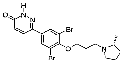
6-{3,5-Dibromo-4-[3-(( R )-2-methyl-pyrrolidin-1-yl)-propoxy]-phenyl}-2H-pyridazin-3-one
