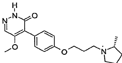
5-Methoxy-4-{4-[3-((R)-2-methyl-pyrrolidin-1-yl)-propoxy]-phenyl}-2H-pyridazin-3-one
