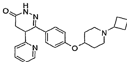
6-[4-(1-Cyclobutyl-piperidin-4-yloxy)-phenyl]-5-pyridin-2-yl-4,5-dihydro-2H-pyridazin-3-one
