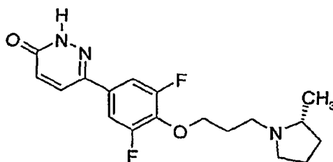
6-{3,5-Difluoro-4-[3-((R)-2-methylpyrrolidin-1-yl)-propoxy]-phenyl}-2H-pyridazin-3-one
