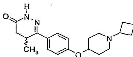
6-[4-(1-Cyclobutyl-piperidin-4-yloxy)-phenyl] -5-methyl-4,5-dihydro-2H-pyridazin-3-one
