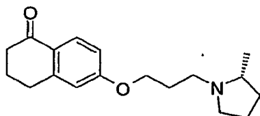
6-[3-((R)-2-Methyl-pyrrolidin-1-yl)-propoxy]-3,4-dihydro-2H-naphthalen-1-one
