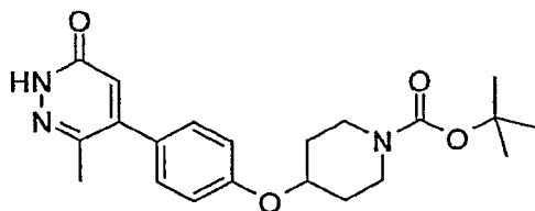
4-[4-(3-Methyl-6-oxo-1,6-dihydro-pyridazin-4-yl)-phenoxy]-piperidine-1-carboxylic acid tert-butyl ester
