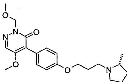
5-Methoxy-2-methoxymethyl-4-{4-[3-((R)-2-methyl-pyrrolidin-1-yl)-propoxy]-phenyl}-2H-pyridazin-3-one
