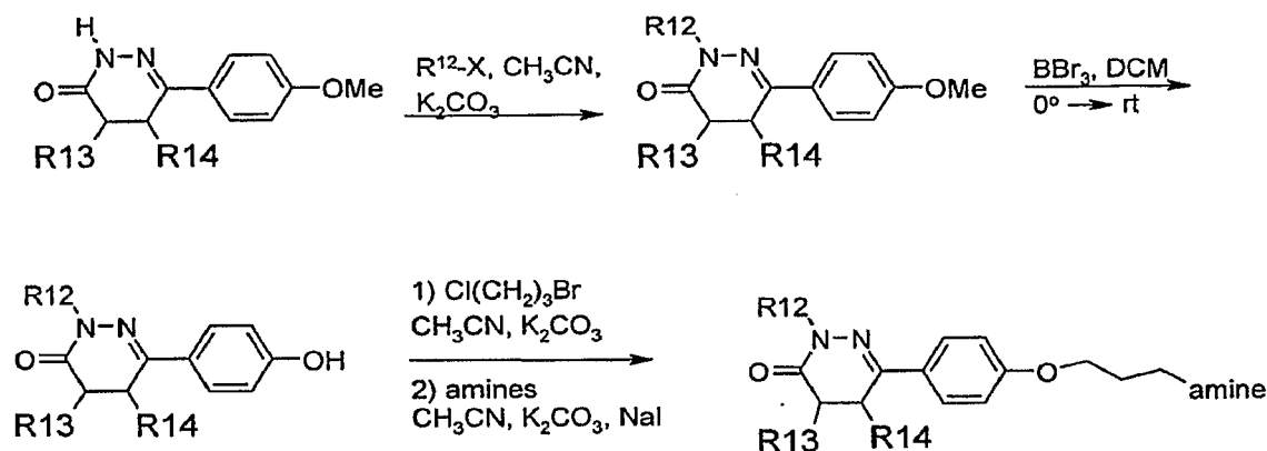
Scheme 2. General synthesis of 4,5-dihydro examples
