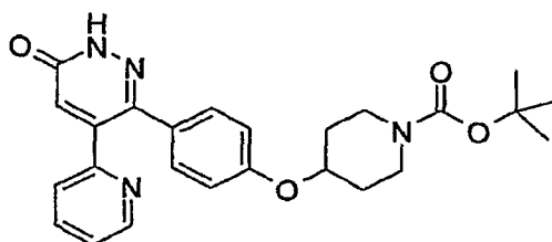
4-[4-(6-Oxo-4-pyridin-2-yl-1,6-dihydro-pyridazin-3-yl)-phenoxy]-piperidine-1-carboxylic acid tert-butyl ester
