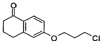
6-(3-Chloro-propoxy)-3,4-dihydro-2H-naphthalen-1-one
