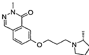
2-Methyl-7-[3-((R)-2-methyl-pyrrolidin-1-yl)-propoxy]-2H-phthalazin-1-one
