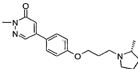
2-Methyl-5-{4-[3-((R)-2-methyl-pyrrolidin-1-yl)-propoxy]-phenyl}-2H-pyridazin-3-one
