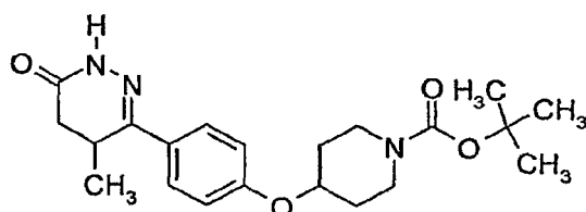
4-[4-(4-Methyl-6-oxo-1,4,5,6-tetrahydro-pyridazin-3-yl)-phenoxy]-piperidine-1-carboxylic acid tert-butyl ester
