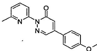
5-(4-Methoxy-phenyl)-2-(6-methyl-pyridin-2-yl)-2H-pyridazin-3-one
