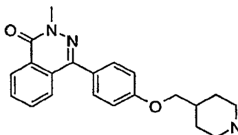
2-Methyl-4-[4-(piperidin-4-ylmethoxy)-phenyl]-2H-phthalazin-1-one
