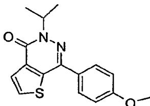
5-Isopropyl-7-(4-methoxy-phenyl)-5H -thieno[2,3-d]pyridazin-4-one
