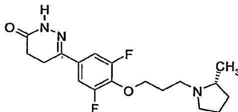
6-{3,5-Difluoro-4-[3-(( R )-2-methyl-pyrrolidin-1-yl)-propoxy]-phenyl}-4,5-dihydro-2H-pyridazin-3-one
