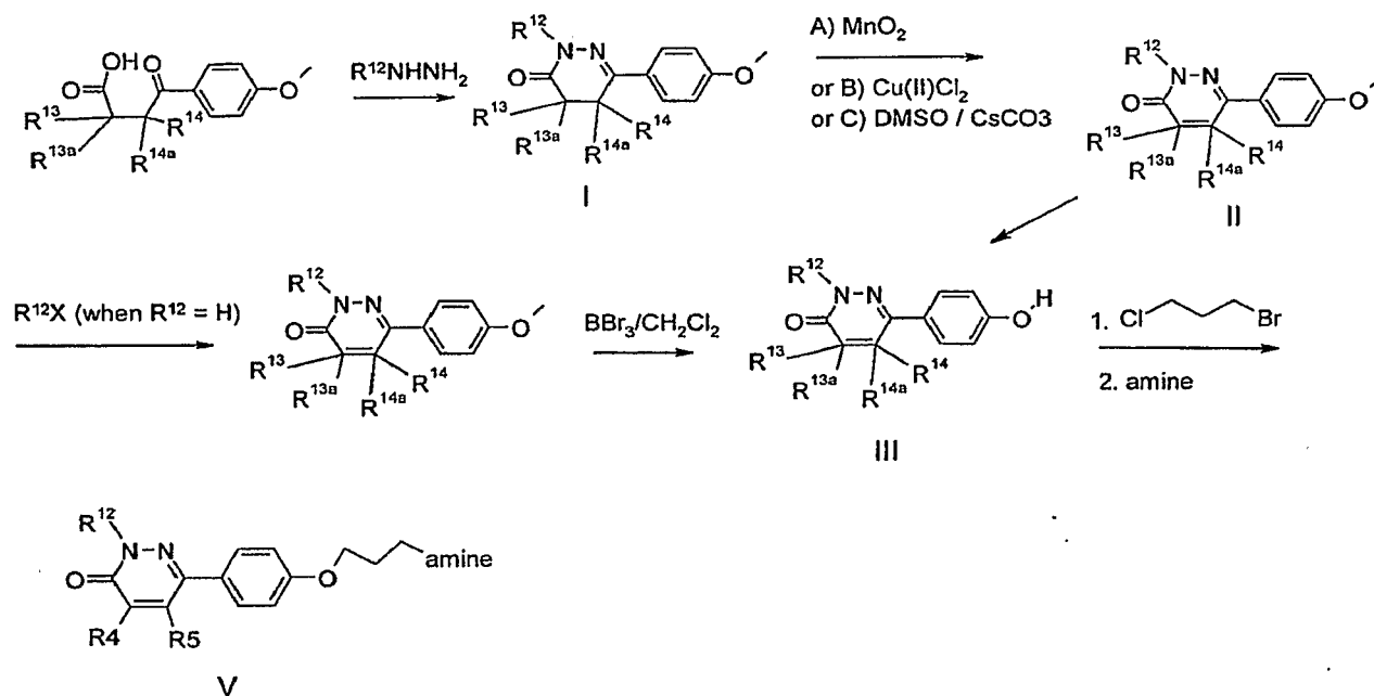
Scheme 3. General synthesis of R 12 H and substituted examples
