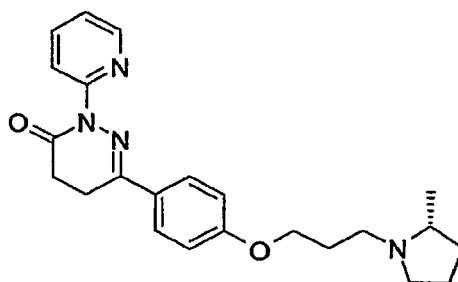
6-[4-[3-((R)-2-Methyl-pyrrolidin-1-yl)-propoxy]-phenyl]-2-pyridin-2-yl-4,5-dihydro-2H-pyridazin-3-one
