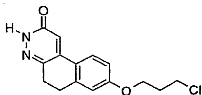
8-(3-Chloro-propoxy)-5,6-dihydro-3H-benzo[f]cinnolin-2-one
