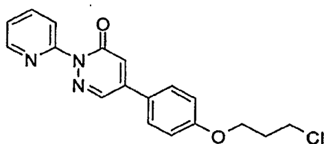
5-[4-(3-Chloro-propoxy)-phenyl]-2-pyridin-2-yl-2H-pyridazin-3-one
