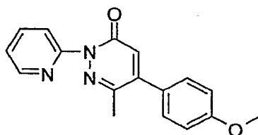
5-(4-Methoxy-phenyl)-6-methyl-2-pyridin-2-yl-2H-pyridazin-3-one
