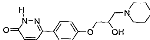
6-[4-(2-Hydroxy-3-piperidin-1-yl-propoxy)-phenyl]-2H-pyridazin-3-one
