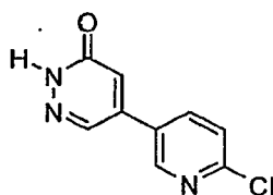
5-(6-Chloro-pyridin-3-yl)-2H- pyridazin-3-one
