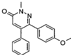
6-(4-Methoxy-phenyl)-2-methyl-5-phenyl-2H-pyridazin-3-one
