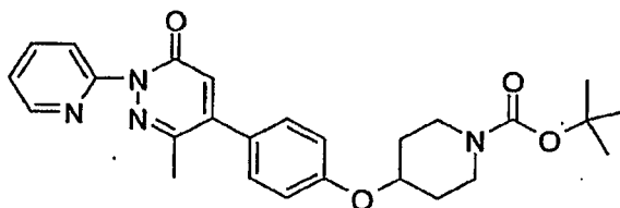
4-[4-(3-Methyl-6-oxo-1-pyridin-2-yl-1,6-dihydro-pyridazin-4-yl)-phenoxyl]-piperidine-1-carboxylic acid tert-butyl ester
