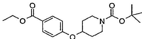
4-(4-Ethoxycarbonyl-phenoxy)-piperidine-1-carboxylic acid tert-butyl ester
