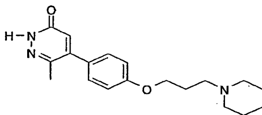
6-Methyl-5-[4-(3-piperidin-1-yl-propoxy)-phenyl]-2H-pyridazin-3-one
