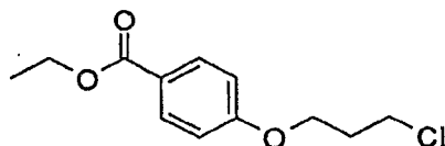
4-(3-Chloro-propoxy)-benzoic acid ethyl ester
