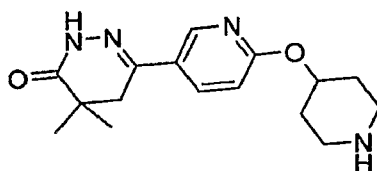
4,4-Dimethyl-6-[6-(piperidin-4-yloxy)-pyridin-3-yl]-4,5-dihydro-2H-pyridazin-3-one
