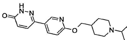
6-[6-(1-isopropyl-piperidin-4-ylmethoxy)- pyridin-3-yl]-2H-pyridazin-3-one
