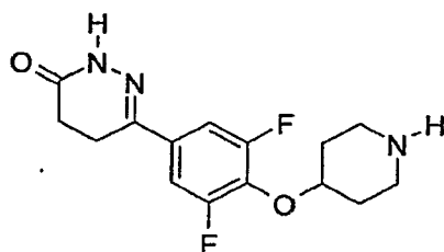
6-[3,5-Difluoro-4-(piperidin-4-yloxy)-phenyl]-4,5-dihydro-2H-pyridazin-3-one
