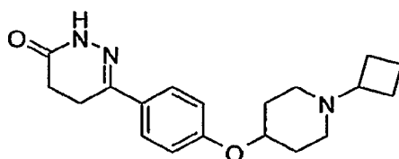
6-[4-(1-Cyclobutyl-piperidin-4-yloxy)-phenyl]-4,5-dihydro-2H-pyridazin-3-one
