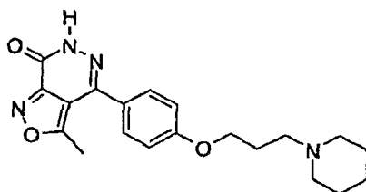
3-Methyl-4-[4-(3-piperidin-1-yl-propoxy)-phenyl]-6H-isoxazolo[3,4-d]pyridazin-7-one
