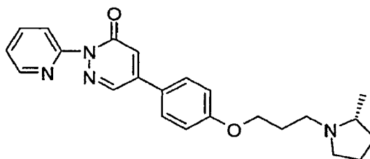
5-{4-[3-((R)-2-Methyl-pyrrolidin-1-yl)-propoxy]-phenyl}-2-pyridin-2-yl-2H-pyridazin-3-one
