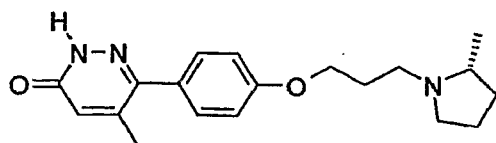
5-Ethyl-6-{4-[3-((R)-2-methyl-pyrrolidin-1-yl)-propoxy]-phenyl}-2H-pyridazin-3-one
