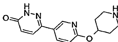
6-[6-(Piperidin-4-yloxy)-pyridin-3-yl]-2H-pyridazin-3-one
