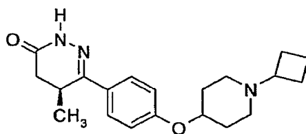
(S)-6-[4-(1-Cyclobutyl-piperidin-4-yloxy)-phenyl]-5-methyl-4,5-dihydro-2H-pyridazin-3-one
