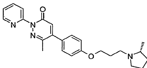
6-Methyl-5-{4-[3-((R)-2-methyl-pyrrolidin-1-yl)-propoxy]-phenyl}-2-pyridin-2-yl-2H-pyridazin-3-one
