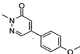
5-(4-Methoxy-phenyl)-2-methyl-2H-pyridazin-3-one
