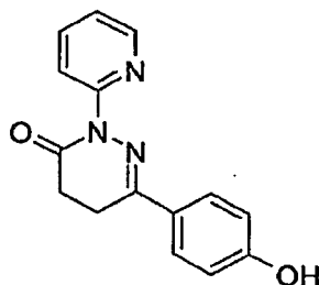
6-(4-Hydroxy-phenyl)-2-pyridin-2-yl-4,5-dihydro-2H-pyridazin-3-one
