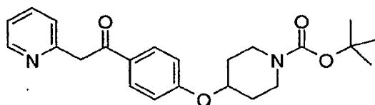
4-[4-(2-Pyridin-2-yl-acetyl)-phenoxy]piperidine-1-carboxylic acid tert-butyl ester
