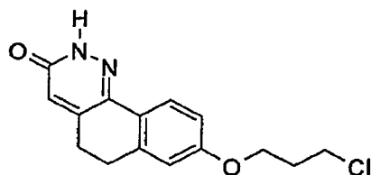
8-(3-Chloro-propoxy)-5,6-dihydro-2H-benzo[h]cinnolin-3-one
