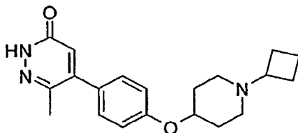
5-[4-(1-Cyclobutyl-piperidin-4-yloxy)-phenyl]-6-methyl-2H-pyridazin-3-one
