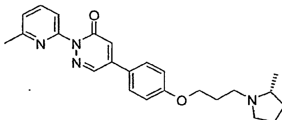
2-(6-Methyl-pyridin-2-yl)-5-{4-[3-((R)-2-methyl-pyrrolidin-1-yl)-propoxy]-phenyl}-2H-pyridazin-3-one
