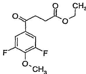
4-(3,5-Difluoro-4-methoxy-phenyl)-4-oxo-butanoic acid ethyl ester
