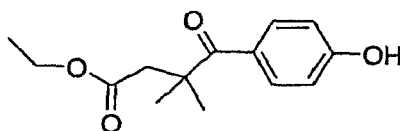
4-(4-Hydroxy-phenyl)-3,3-dimethyl-4 -oxo-butanoic acid ethyl ester
