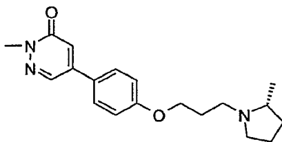
2-Methyl-5-{4-[3-((R)-2-methyl-pyrrolidin-1-yl)-propoxy]-phenyl}-2H-pyridazin-3-one
