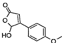
5-Hydroxy-4-(4-methoxy-phenyl)-5H-furan-2-one
