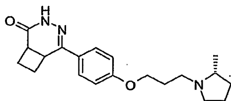
5-{4-[3-((R)-2-Methyl-pyrrolidin-1-yl)-propoxy]-phenyl}-3,4-diazabicyclo[4.2.0]oct-4-en-2-one
