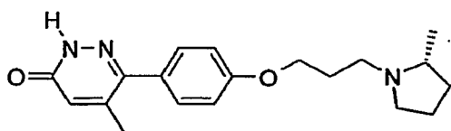
5-Methyl-6-{4-[3-((R)-2-methyl-pyrrolidin-1-yl)-propoxy]-phenyl}-2H-pyridazin-3-one
