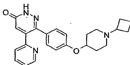
6-[4-(1-Cyclobutyl-piperidin-4-yloxy)-phenyl]-5-pyridin-2-yl-2H-pyridazin-3-one
