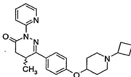
6-[4-(1-Cyclobutyl-piperidin-4-yloxy)-phenyl]-5-methyl-2-pyridin-2-yl-4,5-dihydro-2H-pyridazin-3-one
