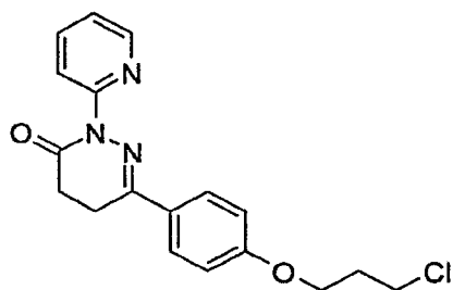
6-[4-(3-Chloro-propoxy)-phenyl]-2-pyridin-2-yl-4,5-dihydro-2H-pyridazin-3-one
