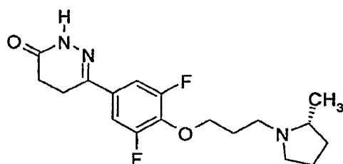
6-{3,5-Difluoro-4-[3-(( R )-2-methyl-pyrrolidin-1-yl)-propoxy]-phenyl}-4,5-dihydro-2H-pyridazin-3-one
