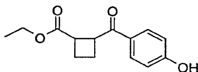
2-(4-Hydroxy-benzoyl)-cyclobutanecarboxylic acid ethyl ester
