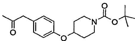
4-[4-(2-Oxo-propyl)-phenoxy]-piperidine-1-carboxylic acid tert-butyl ester
