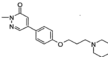
2-Methyl-5-[4-(3-piperidin-1-yl-propoxy)-phenyl]-2H-pyridazin-3-one
