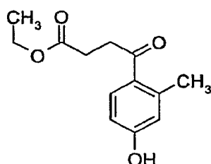
4-(4-Hydroxy-2-methyl-phenyl)-4-oxo-butanoic acid ethyl ester
