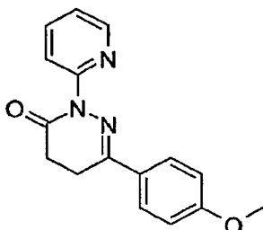
6-(4-Methoxy-phenyl)-2-pyridin-2-yl-4,5-dihydro-2H-pyridazin-3-one
