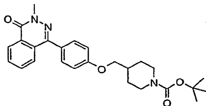
4-[4-(3-Methyl-4-oxo-3,4-dihydro-phthalazin-1-yl)-phenoxy]methyl-piperidine-1-carboxylic acid tert-butyl ester
