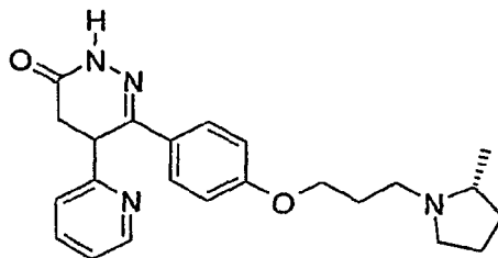
6-{4-[3-((R)-2-Methyl-pyrrolidin-1-yl)-propoxy]-phenyl}-5-pyridin-2-yl-4,5-dihydro-2H-pyridazin-3-one
