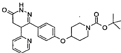
4-[4-(6-Oxo-4-pyridin-2-yl-1,4,5,6-tetrahydro-pyridazin-3-yl)-phenoxy]-piperidine-1-carboxylic acid tert-butyl ester
