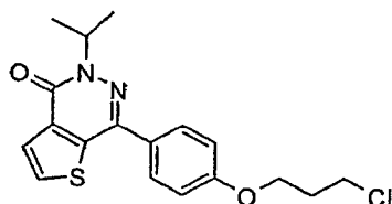
7-[4-(3-Chloro-propoxy)-phenyl]-5-isopropyl-5H-thieno[2,3-d]pyridazin-4-one
