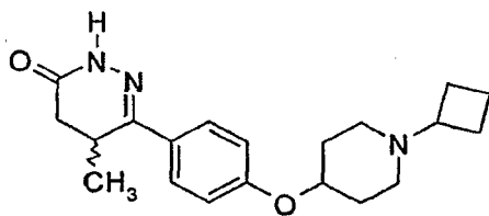
6-[4-(1-Cyclobutyl-piperidin-4-yloxy)-phenyl]-5-methyl-4,5-dihydro-2H-pyridazin-3-one
