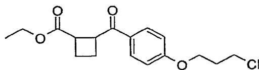
2-[4-(3-Chloro-propoxy)-benzoyl]-cyclobutanecarboxylic acid ethyl ester
