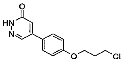
5-[4-(3-Chloro-propoxy)-phenyl]-2H-pyridazin-3-one
