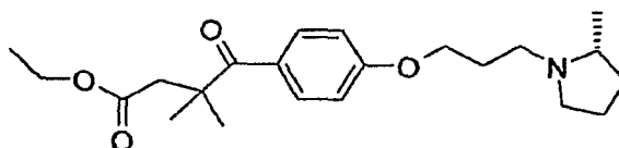
3,3-Dimethyl-4-{4-[3-((R)-2-methylpyrrolidin-1-yl)propoxy]phenyl}-4-oxo-butyric acid ethyl ester
