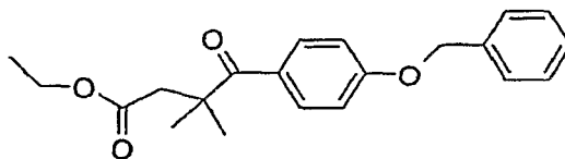
4-(4-Benzyloxy-phenyl)-3,3-dimethyl -4-oxo-butanoic acid ethyl ester
