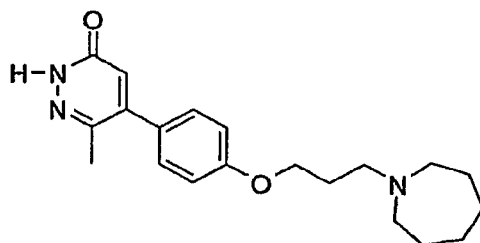
5-[4-(3-Azepan-1-yl-propoxy)-phenyl]-6-methyl-2H-pyridazin-3-one
