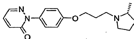
2-{4-[3-((R)-2-Methyl-pyrrolidin-1-yl)-propoxy]-phenyl}-2H-pyridazin-3-one
