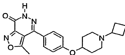
4-[4-(1-Cyclobutyl-piperidin-4-yloxy)-phenyl]-3-methyl-6H-isoxazolo[3,4-d]pyridazin-7-one
