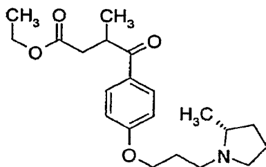
3-Methyl-4-{4-[3-((R)-2-methyl-pyrrolidin-1-yl)-propoxy]-phenyl}-4-oxo-butyric acid ethyl ester
