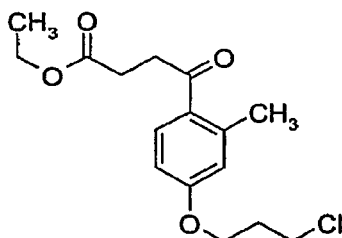
4-(4-(3-Chloro-propoxy)-2-methyl-phenyl)-4-oxo-butanoic acid ethyl ester
