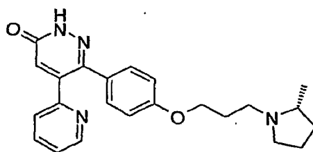
6-{4-[3-((R)-2-Methyl-pyrrolidin-1-yl)-propoxy]-phenyl}-5-pyridin-2-yl-2H-pyridazin-3-one
