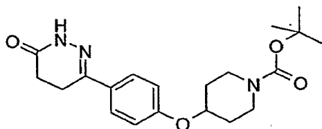
4-[4-(6-Oxo-1,4,5,6-tetrahydro-pyridazin-3-yl)-phenoxy]-piperidine-1-carboxylic acid tert-butyl ester
