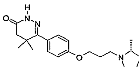
5,5-Dimethyl-6-{4-[3-((R)-2-methylpyrrolidin-1-yl)propoxy]phenyl}-4,5-dihydro-2H-pyridazin-3-one
