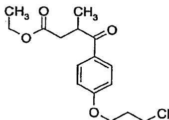
4-[4-(3-Chloro-propoxy)-phenyl]-3-methyl-4-oxo-butyric acid ethyl ester
