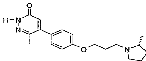
6-Methyl-5-{4-[3-((R)-2-methyl-pyrrolidin-1-yl)-propoxy]-phenyl}-2H-pyridazin-3-one
