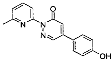
5-(4-Hydroxy-phenyl)-2-(6-methyl-pyridin-2-yl)-2H-pyridazin-3-one
