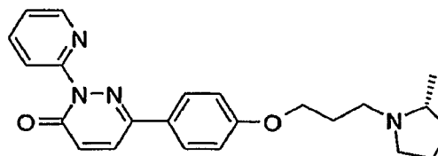
6-{4-[3-((R)-2-Methyl-pyrrolidin-1-yl)-propoxy]-phenyl}-2-pyridin-2-yl-2H-pyridazin-3-one
