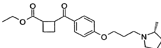
2-[4-[3-((R)-2-Methyl-pyrrolidin-1-yl)-propoxy]-benzoyl]-cyclobutanecarboxylic acid ethyl ester
