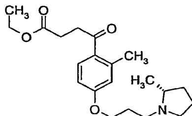
4-{2-Methyl-4-[3-((R)-2-methyl-pyrrolidin-1-yl)-propoxy]-phenyl}-4-oxo-butyrac acid ethyl ester
