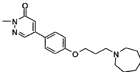
5-[4-(3-Azepan-1-yl-propoxy)-phenyl]-2-methyl-2H-pyridazin-3-one
