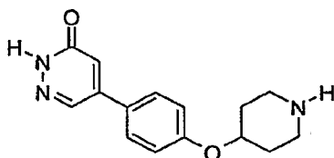
5-[4-(Piperidin-4-yloxy)-phenyl]-2H-pyridazin-3-one
