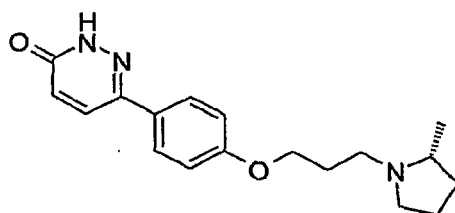
6-[4-[3-((R)-2-Methyl-pyrrolidin-1-yl)-propoxy]-phenyl]-2H-pyridazin-3-one
