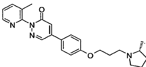
2-(3-Methyl-pyridin-2-yl)-5-{4-[3-((R)-2-methylpyrrolidin-1-yl)-propoxy]-phenyl}-2H-pyridazin-3-one
