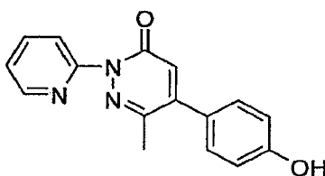
5-(4-Hydroxy-phenyl)-6-methyl-2-pyridin-2-yl-2H-pyridazin-3-one
