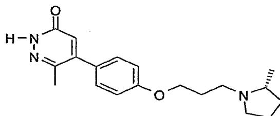
6-Methyl-5-{4-[3-((R)-2-methyl-pyrrolidin-1-yl)-propoxy]-phenyl}-2H-pyridazin-3-one
