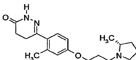
6-((R)-2-Methyl-4-[3-(2-methyl-pyrrolidin-1-yl)-propoxy]-phenyl)-4,5-dihydro-2H-pyridazin-3-one
