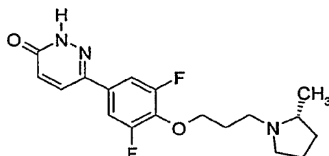
6-{3,5-Difluoro-4-[3-((R)-2-methylpyrrolidin-1-yl)-propoxy]-phenyl}-2H-pyridazin-3-one
