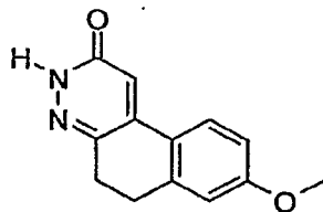
8-Methoxy-5,6-dihydro-3H-benzo[f]cinnolin-2-one
