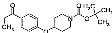
4-(4-Propionyl-phenoxy)-piperidine- 1-carboxylic acid tert-butyl ester
