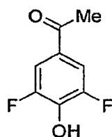
1-(3,5-Difluoro-4-hydroxyphenyl)-ethanone
