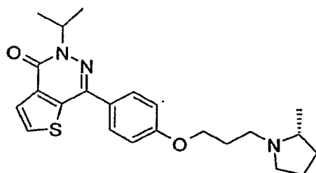
5-Isopropyl-7-{4-[3-((R)-2-methylpyrrolidin-1-yl)-propoxy]-phenyl}-5H-thieno[2,3-d]pyridazin-4-one
