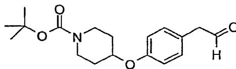
4-[4-(2-Oxo-ethyl)-phenoxy]-piperidine-1-carboxylic acid tert-butyl ester
