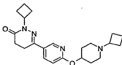
2-Cyclobutyl-6-[6-(1-cyclobutyl-piperidin-4-yloxy)-pyridin-3-yl]-4,5-dihydro-2H-pyridazin-3-one
