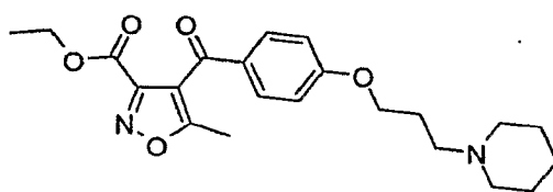
5-Methyl-4-[4-(3-piperidin-1-ylpropoxy)-benzoyl]-isoxazole-3-carboxylic acid ethyl ester
