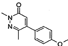
5-(4-Methoxy-phenyl)-2,6-dimethyl-2 H-pyridazin-3-one
