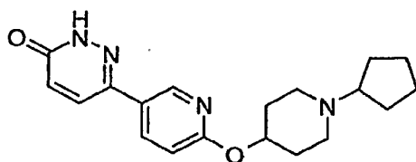
6-[6-(1-Cyclopentyl-piperidin-4-yloxy)-pyridin-3-yl]-2H-pyridazin-3-one
