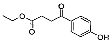
4-(4-Hydroxy-phenyl)-4-oxo-butyric acid ethyl ester
