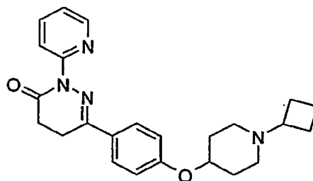
6-[4-(1-Cyclobutyl-piperidin-4-yloxy)-phenyl]-2-pyridin-2-yl-4,5-dihydro-2H-pyridazin-3-one
