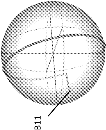
Bloch sphere B11
