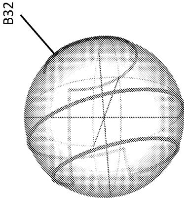
Bloch sphere B32
