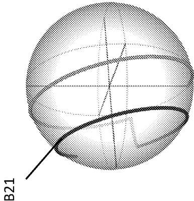
Bloch sphere B21
