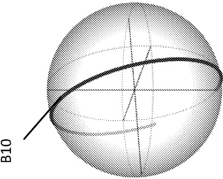
Bloch sphere B10
