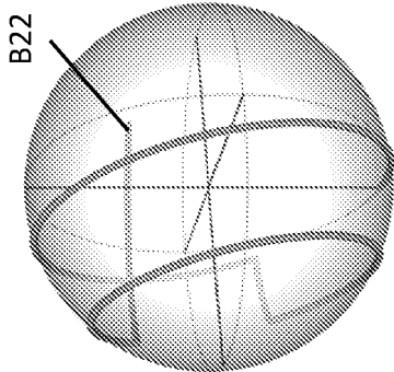
Bloch sphere B22
