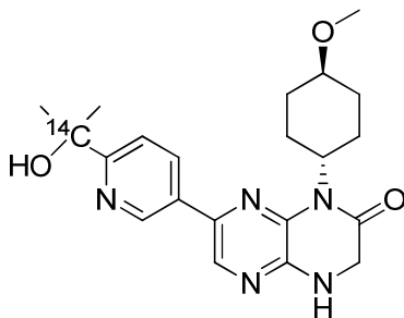
14 C-Compound A
