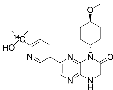
14 C-Compound A
