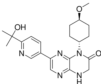
Compound A,
