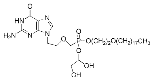
glyceryl octadecyloxyethyl 9-[2-(phosphonomethoxy)ethyl]guanine
