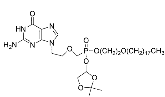
isopropylidenglyceryl octadecyloxyethyl 9-[2-(phosphonomethoxy)ethyl]guanine
