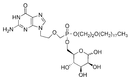
mannosyl octadecyloxyethyl 9-[2-(phosphonomethoxy)ethyl]guanine
