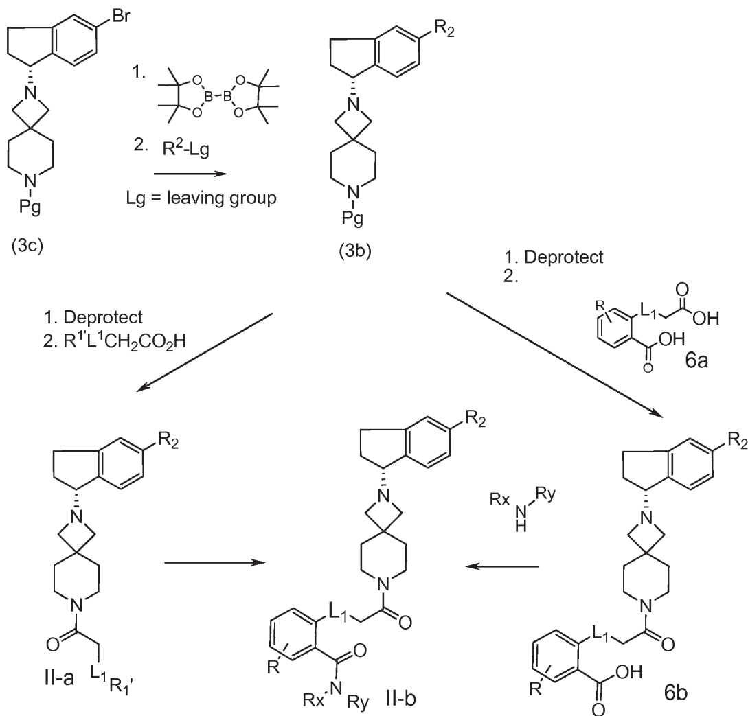
Reaction Scheme VI
