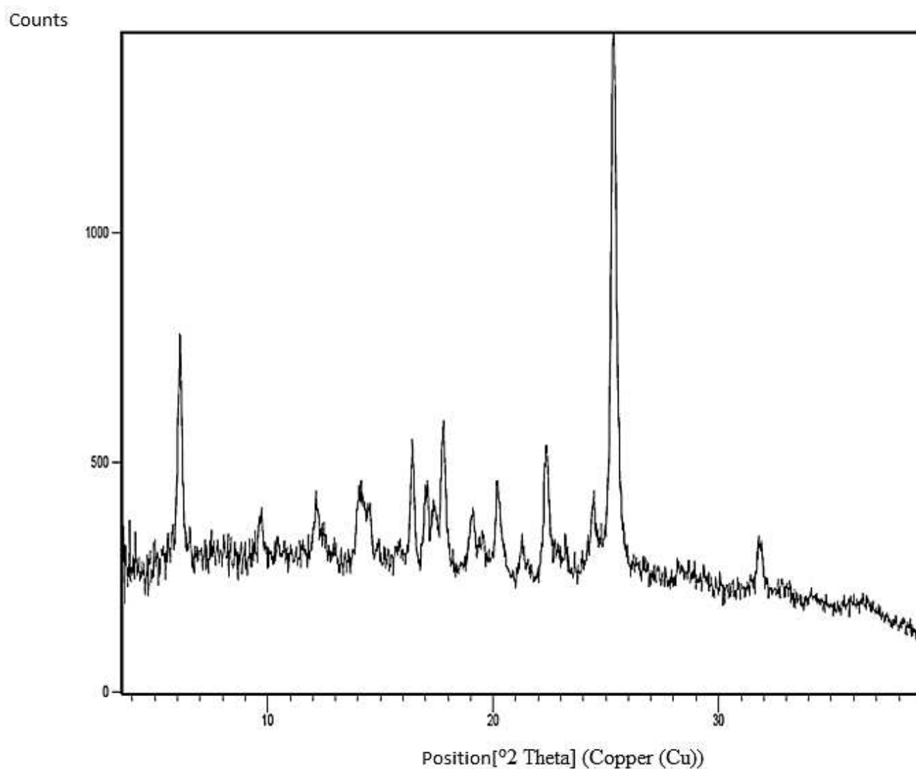
FIGURE 1c: XRPD Compound I-1 (anhydrous form A)
