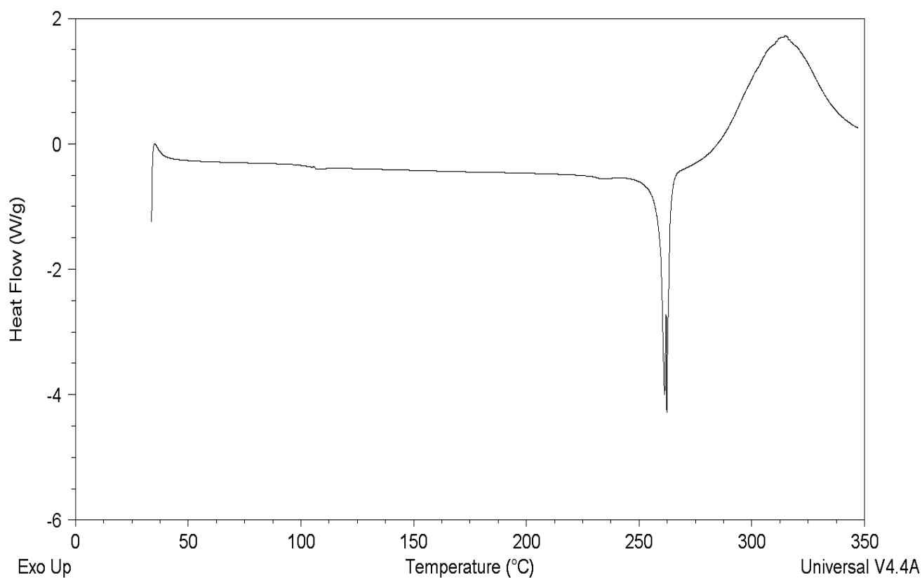
FIGURE 3c: DSC Compound I-1 (anhydrous form A)
