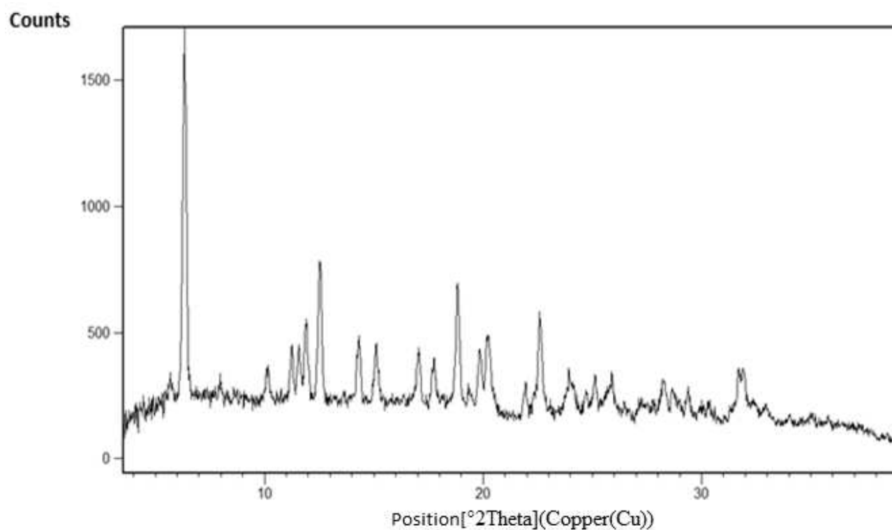
FIGURE 4b: XRPD Compound I-1 (hydrate II)
