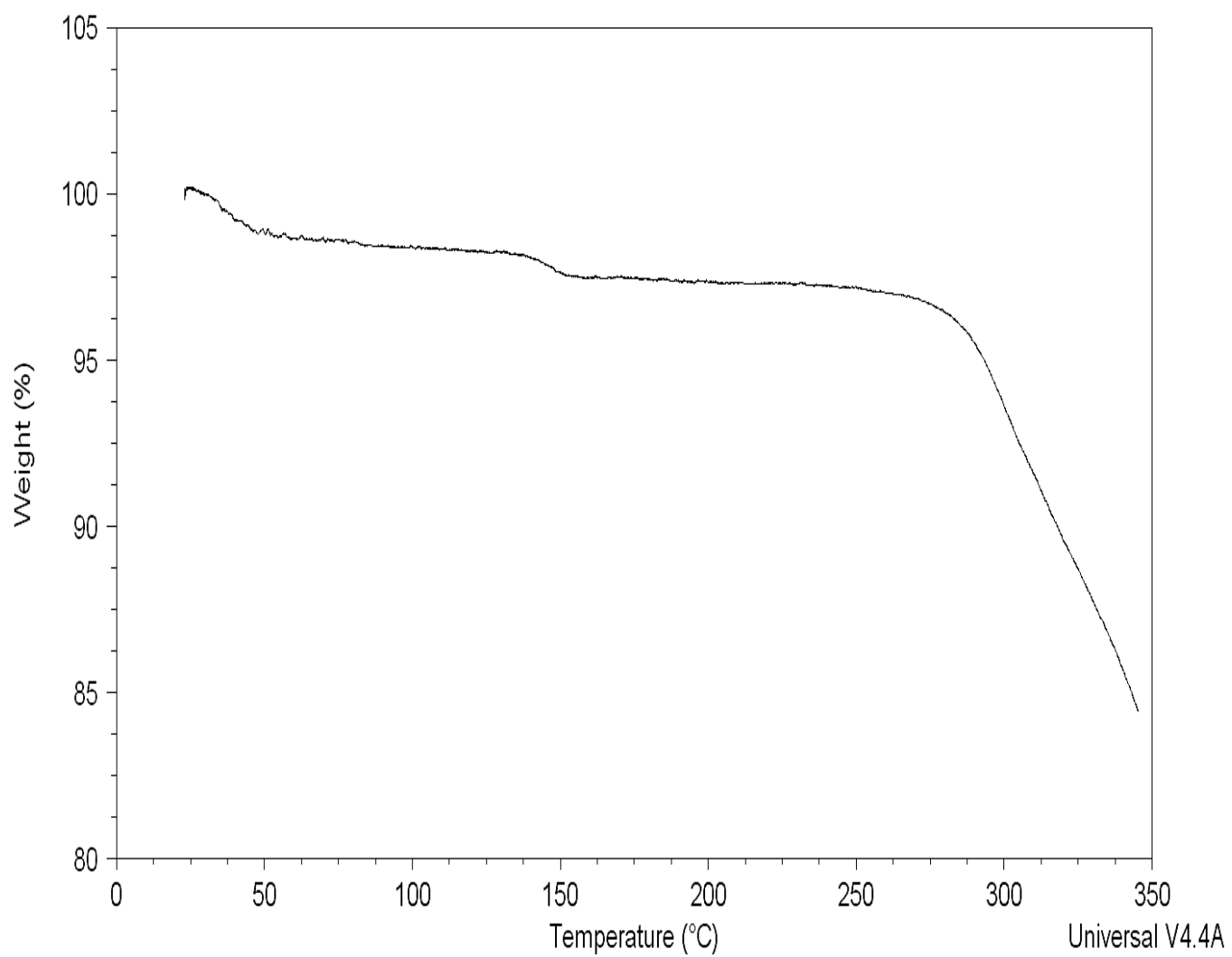
FIGURE 2d: TGA Compound I-1 (anhydrous form B)
