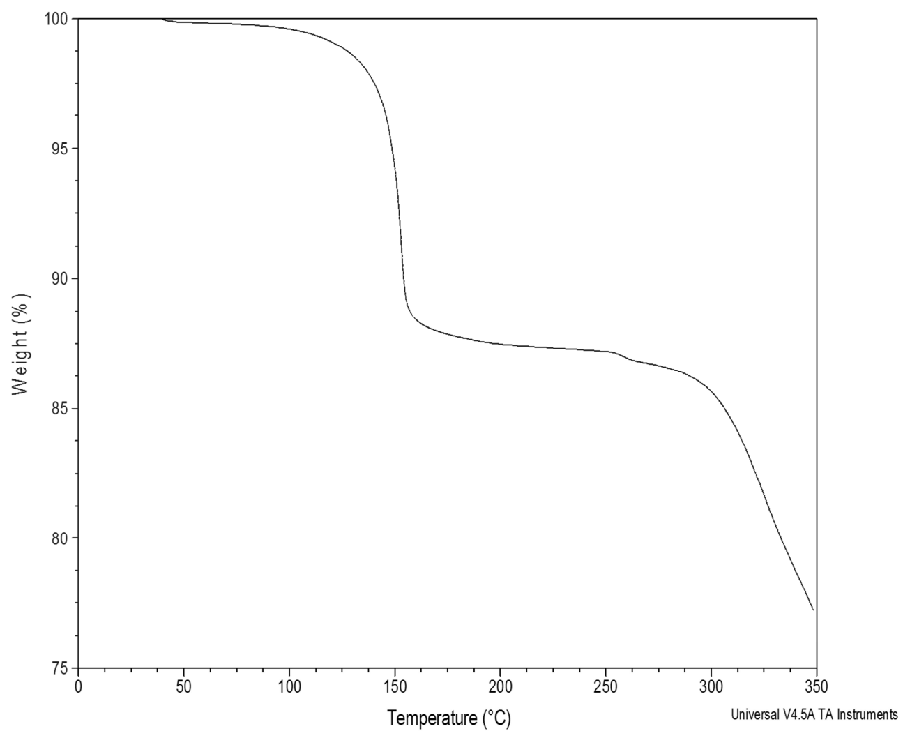
FIGURE 2g: TGA Compound I-1 (DMSO solvate)
