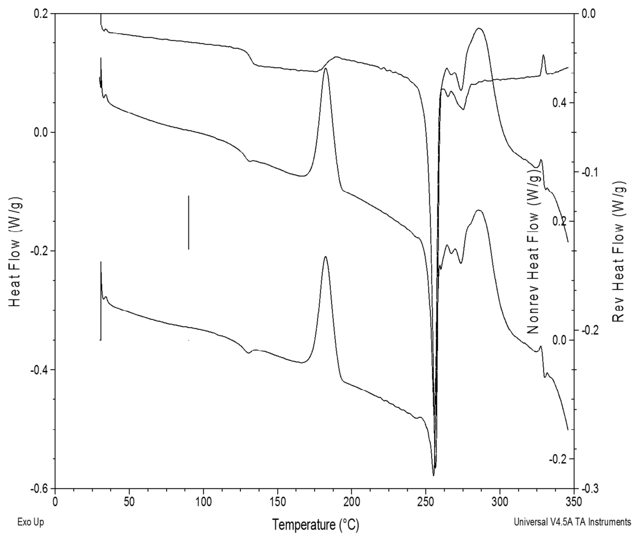
FIGURE 2f: DSC Compound I-1 (amorphous form)
