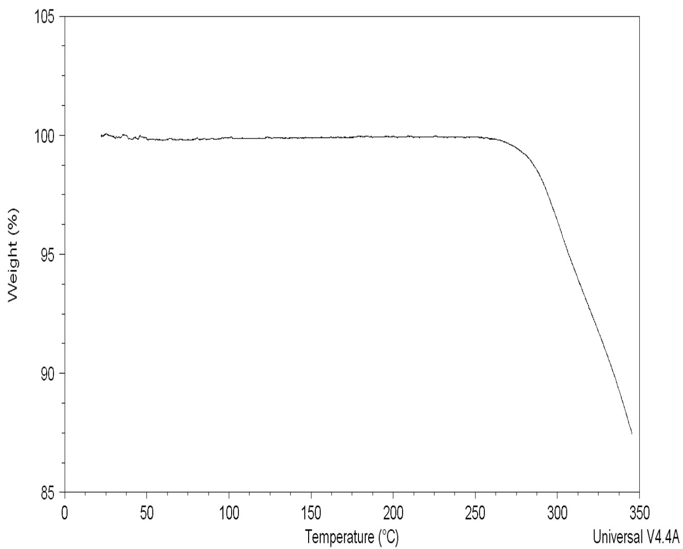
FIGURE 2e: TGA Compound I-1 (anhydrous form C)
