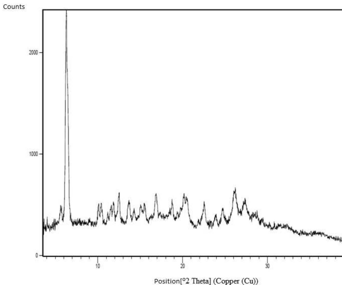
FIGURE 1b: XRPD Compound I-1 (hydrate I)
