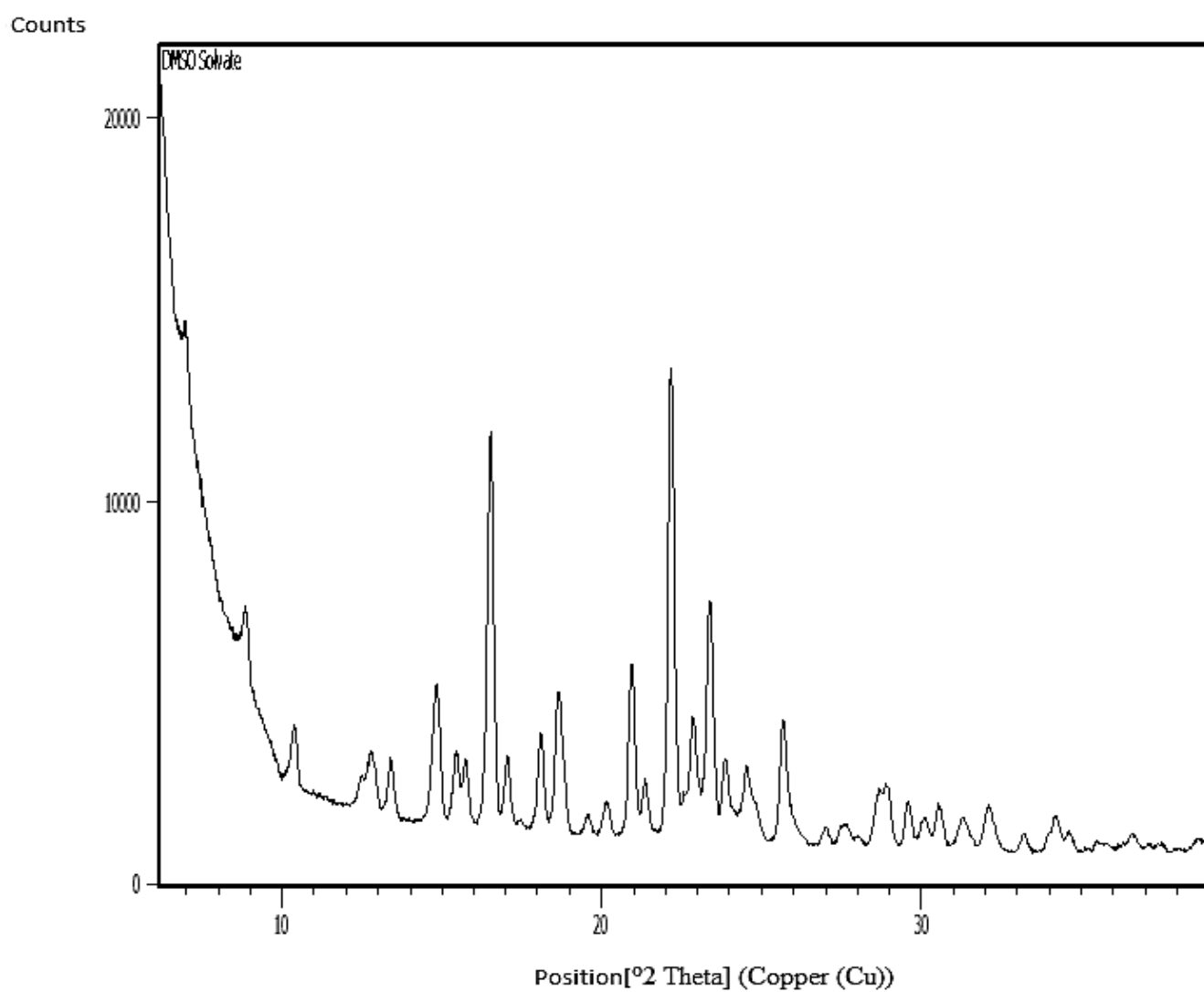
FIGURE 1g: XRPD Compound I-1 (DMSO solvate)
