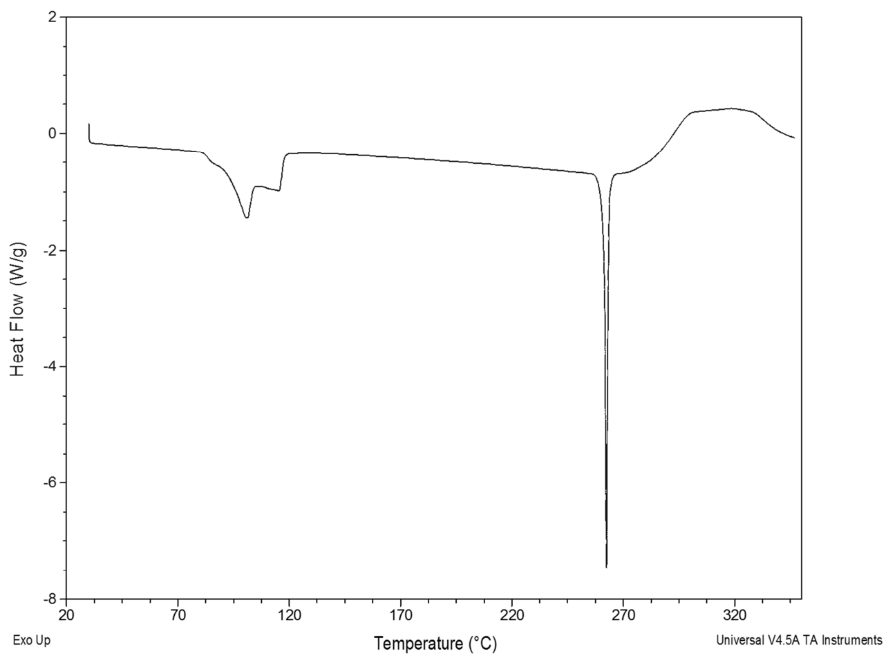
FIGURE 3h: DSC Compound I-1 (DMAC solvate)
