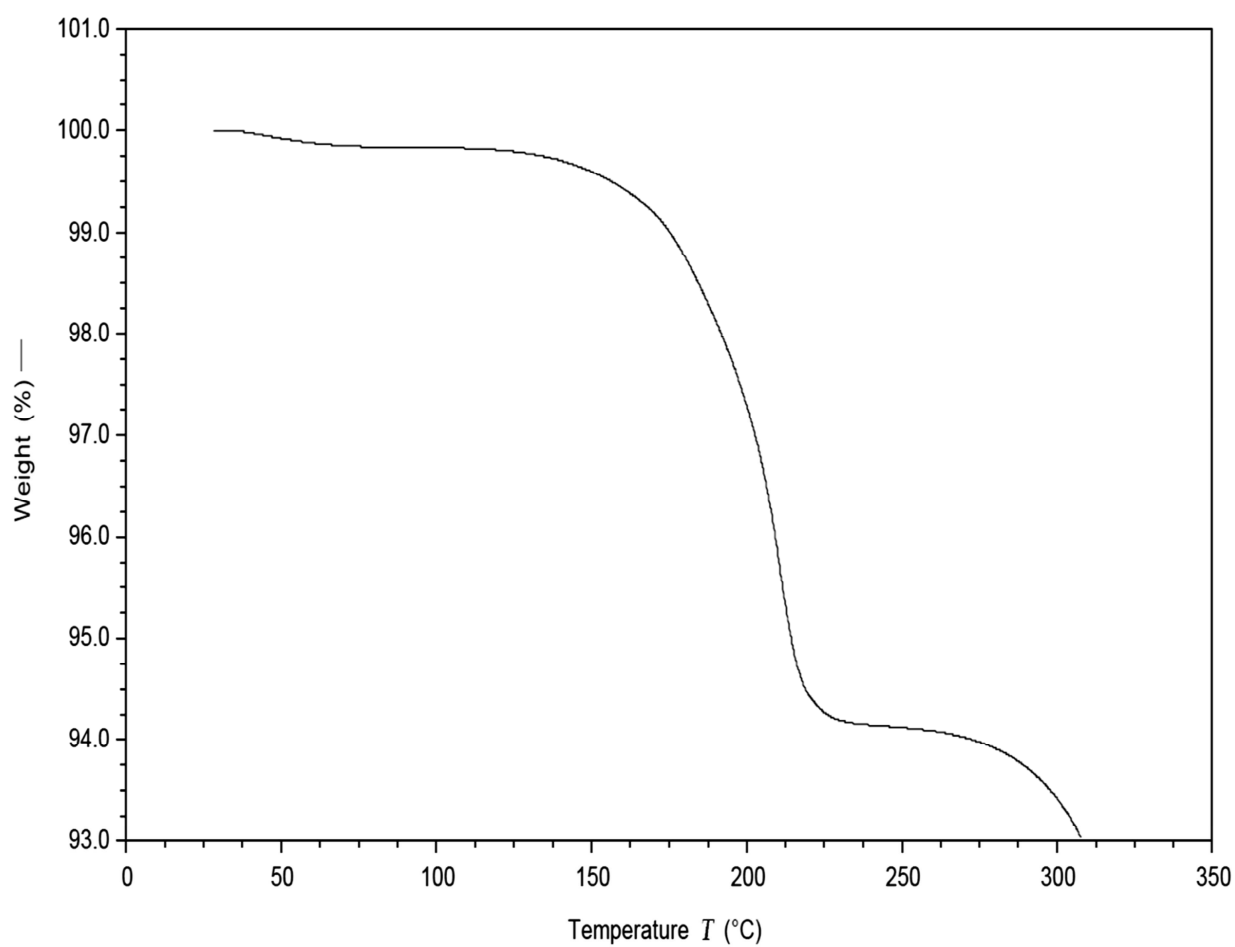
FIGURE 2a: TGA Compound I-1 (ethanol solvate)
