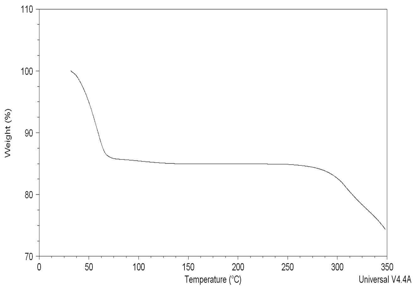
FIGURE 2b: TGA Compound I-1 (hydrate I)
