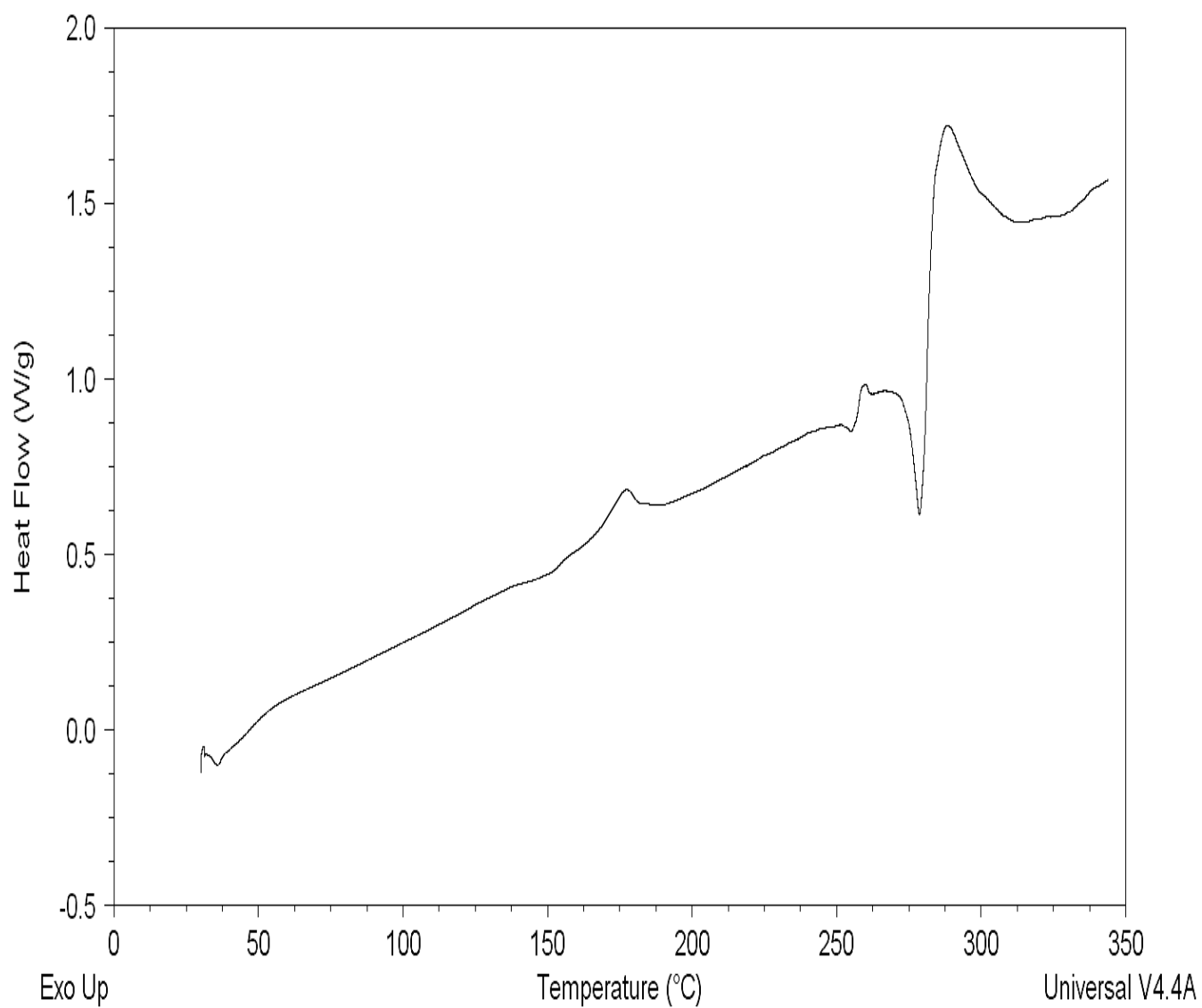
FIGURE 3d: DSC Compound I-1 (anhydrous form B)
