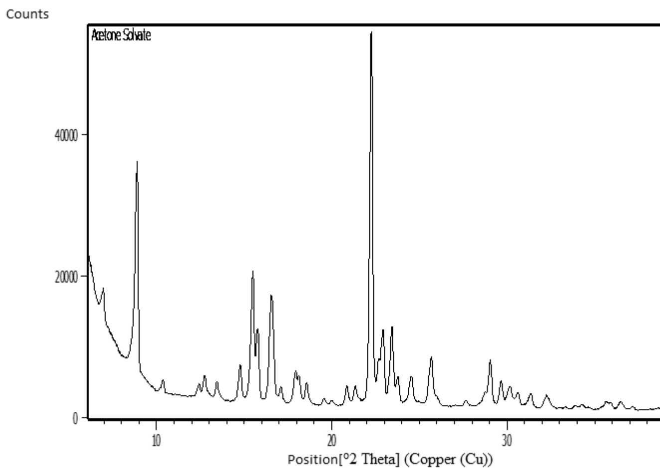
FIGURE 1i: XRPD Compound I-1 (acetone solvate)
