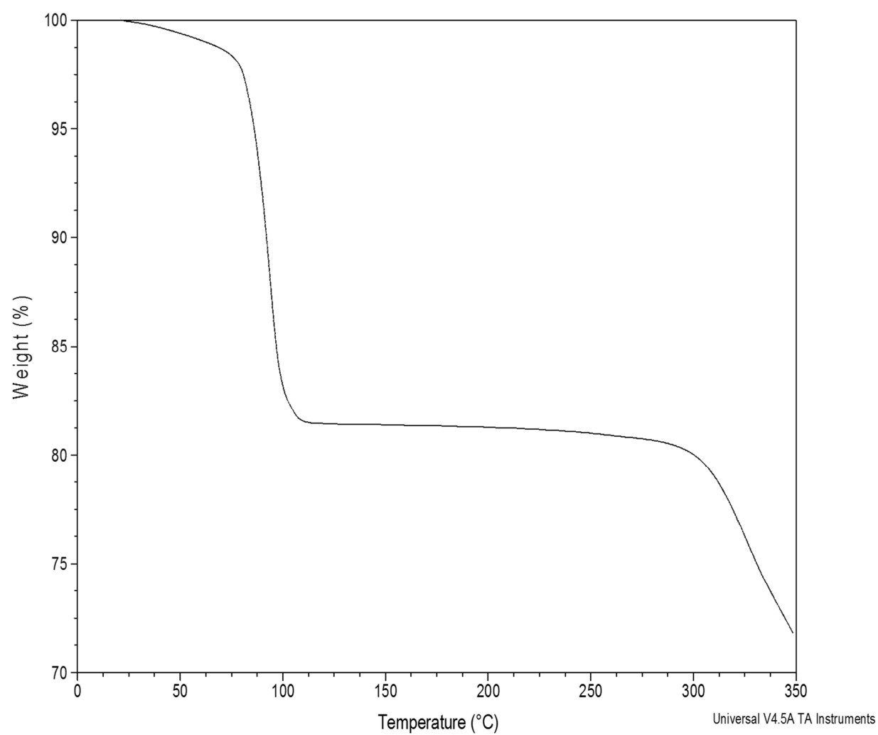
FIGURE 2h: TGA Compound I-1 (DMAC solvate)
