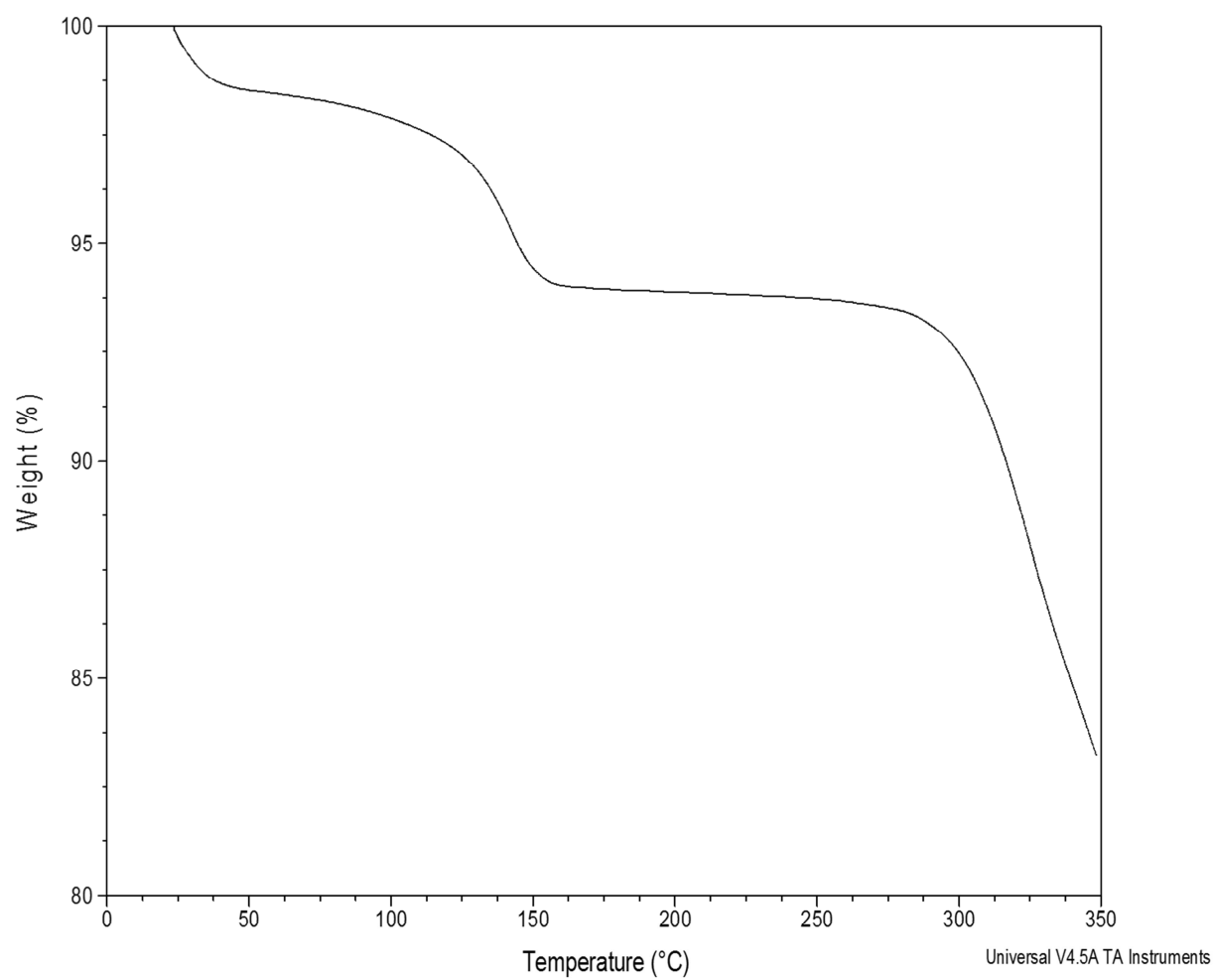
FIGURE 2i: TGA Compound I-1 (acetone solvate)
