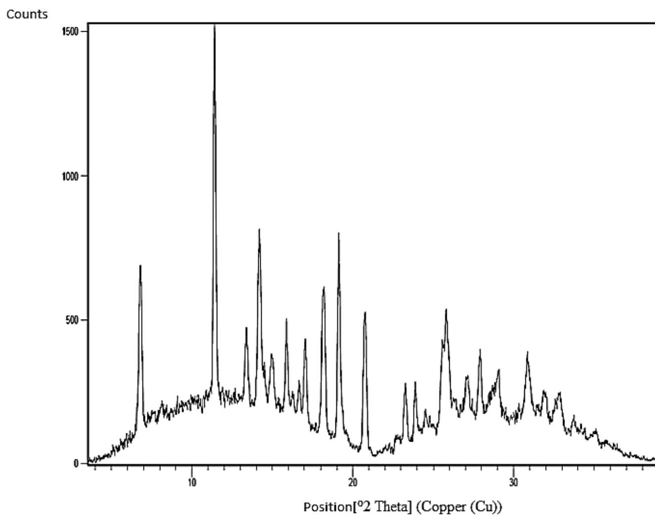
FIGURE 1e: XRPD Compound I-1 (anhydrous form C)
