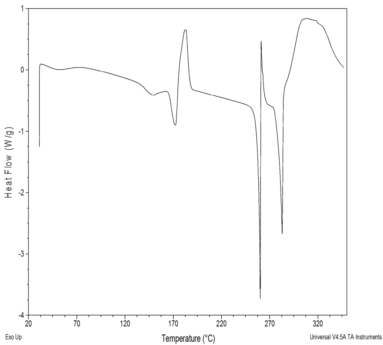
FIGURE 3i: DSC Compound I-1 (acetone solvate)
