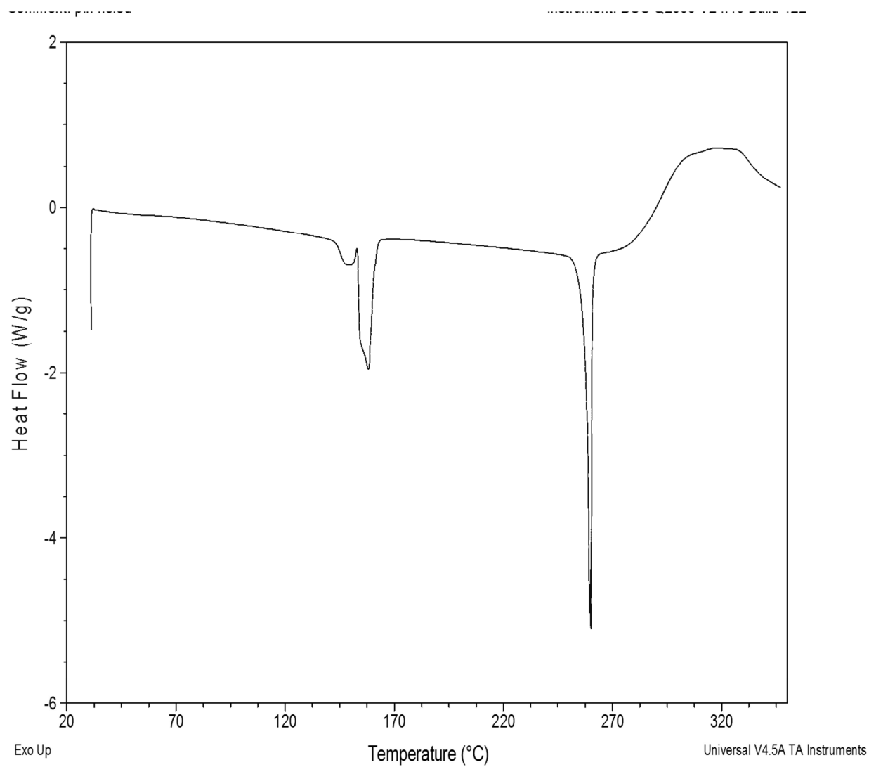
FIGURE 3g: DSC Compound I-1 (DMSO solvate)
