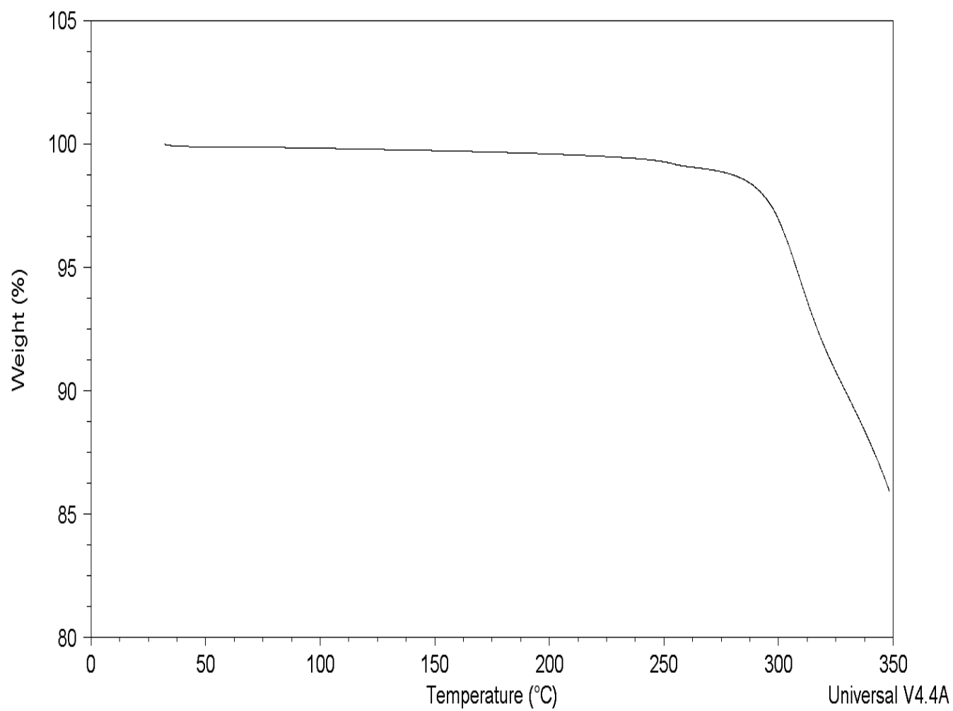
FIGURE 2c: TGA Compound I-1 (anhydrous form A)
