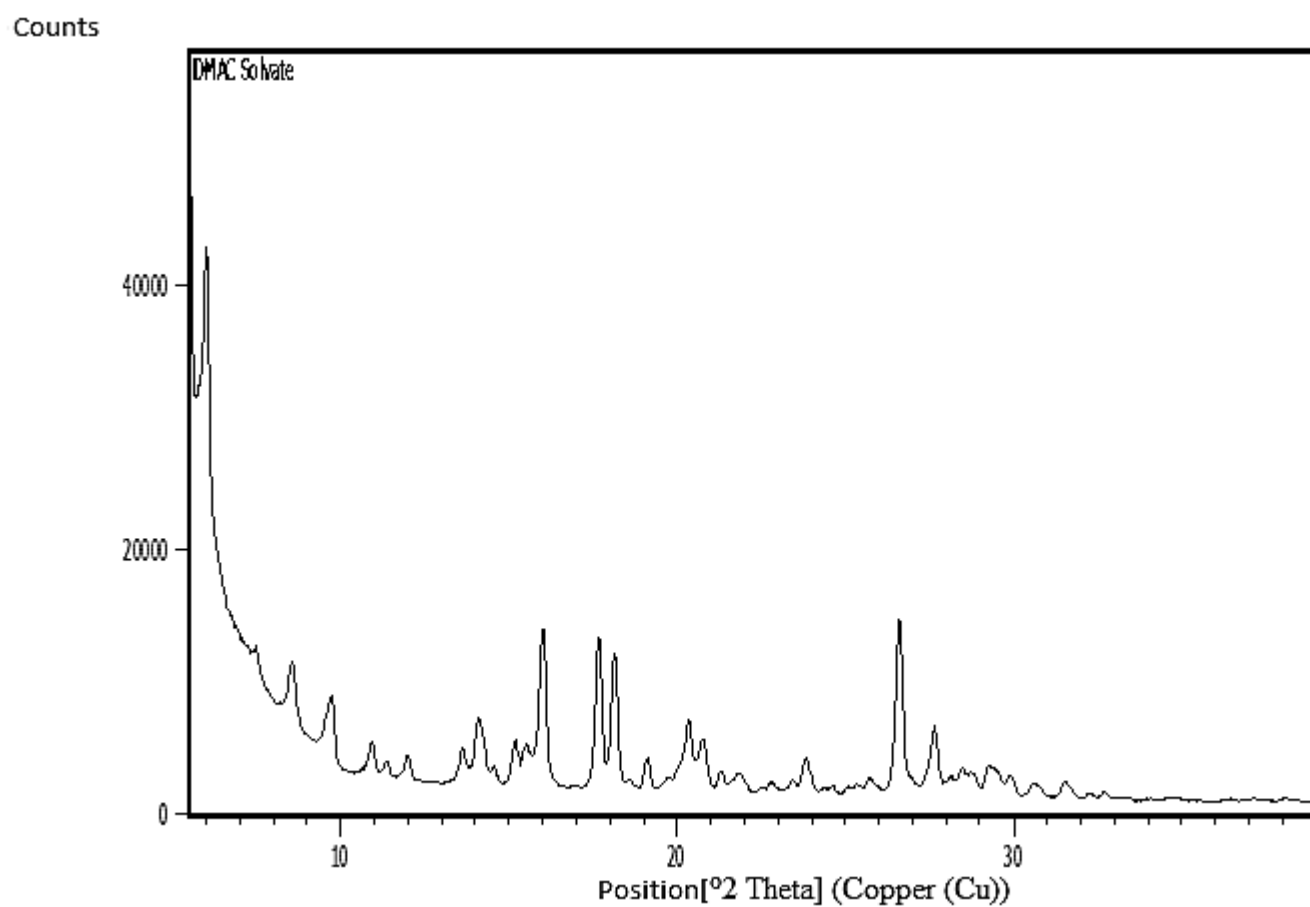
FIGURE 1h: XRPD Compound I-1 (DMAC solvate)
