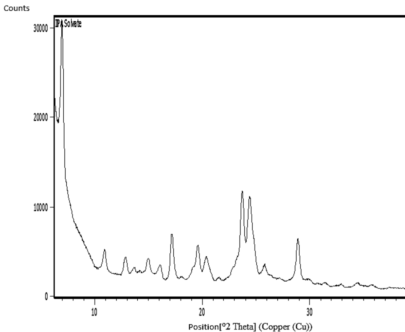
FIGURE 1j: XRPD Compound I-1 (isopropanol solvate)
