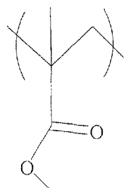
MMA monomer
