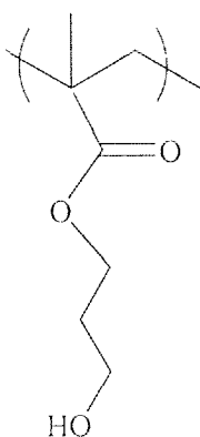
HPMA Monomer
