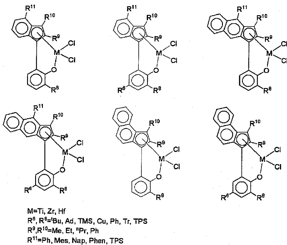
[Chem. 15]
