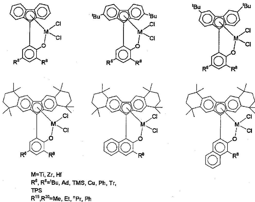
[Chem. 16]
