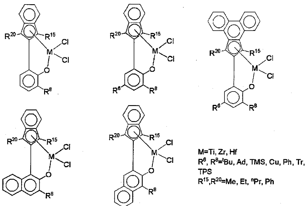
[Chem. 16]
