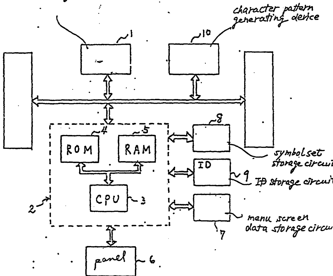
character-code correspondence data storage circuit FIG. 1
