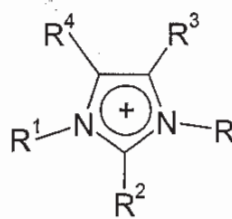
(IVe)
