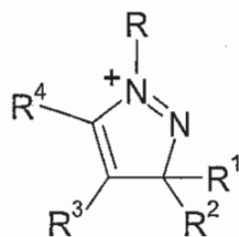
(IVg)
