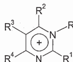
(IVc)
