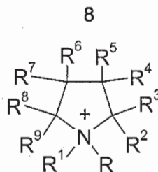
(IVs)
