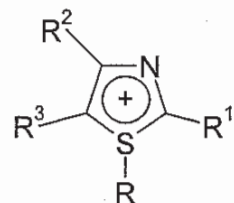
(IVo')
