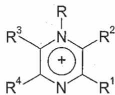
(IVd)
