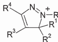
(IVg')
