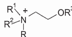
(IVw)
