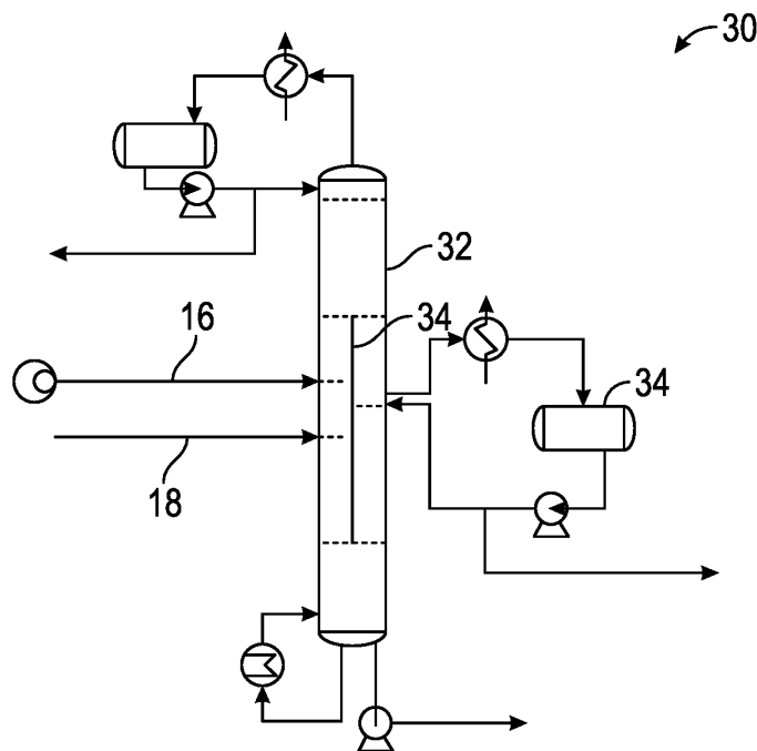
FIG. 2 (PRIOR ART)
