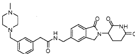
N-((2-(2,6-dioxopiperidin-3-yl)-1-oxoisindolin-5-yl)methyl)-2-(3-((4-methylpiperazin-1-yl)methyl)phenyl)acetamide;
