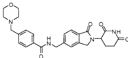
N-((2-(2,6-dioxopiperidin-3-yl)-1-oxoisindolin-5-yl)methyl)-4-(morpholinomethyl)benzamide;
