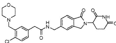
2-(4-chloro-3-(morpholinomethyl)phenyl)-N-((2-(2,6-dioxopiperidin-3-yl)-1-oxoisindolin-5-yl)methyl)acetamide;
