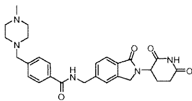
N-((2-(2,6-dioxopiperidin-3-yl)-1-oxoisindolin-5-yl)methyl)-4-((4-methylpiperazin-1-yl)methyl)benzamide;
