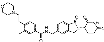
N-((2-(2,6-dioxopiperidin-3-yl)-1-oxoisindolin-5-yl)methyl)-3-methyl-4-(2-morpholinoethyl)benzamide;
