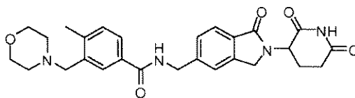
N-((2-(2,6-dioxopiperidin-3-yl)-1-oxoisindolin-5-yl)methyl)-4-methyl-3-(morpholinomethyl)benzamide;
