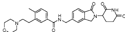
N-((2-(2,6-dioxopiperidin-3-yl)-1-oxoisindolin-5-yl)methyl)-4-methyl-3-(2-morpholinoethyl)benzamide;
