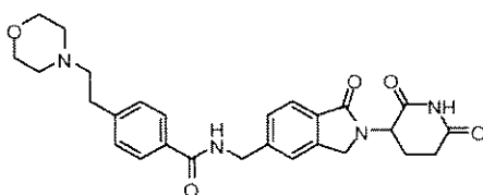
N-((2-(2,6-dioxopiperidin-3-yl)-1-oxoisindolin-5-yl)methyl)-4-(2-morpholinoethyl)benzamide;
