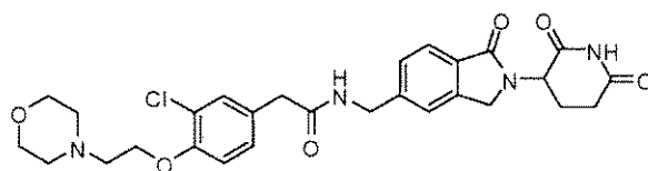
2-(3-chloro-4-(2-morpholinoethoxy)phenyl)-N-((2-(2,6-dioxopiperidin-3-yl)-1-oxoisindolin-5-yl)methyl)acetamide;
