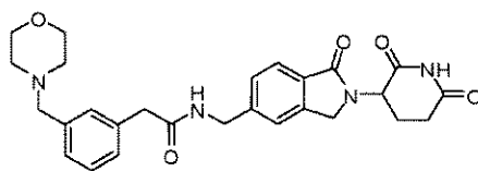
N-((2-(2,6-dioxopiperidin-3-yl)-1-oxoisindolin-5-yl)methyl)-2-(3-(morpholinomethyl)phenyl)acetamide;
