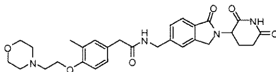
N-((2-(2,6-dioxopiperidin-3-yl)-1-oxoisindolin-5-yl)methyl)-2-(3-methyl-4-(2-morpholinoethoxy)phenyl)acetamide;
