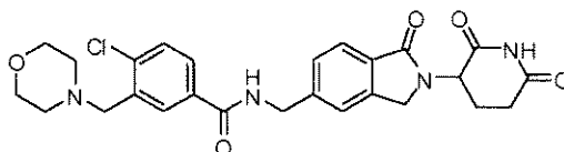
4-chloro-N-((2-(2,6-dioxopiperidin-3-yl)-1-oxoisindolin-5-yl)methyl)-3-(morpholinomethyl)benzamide;
