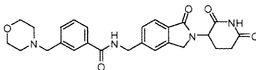
N-((2-(2,6-dioxopiperidin-3-yl)-1-oxoisindolin-5-yl)methyl)-3-(morpholinomethyl)benzamide;
