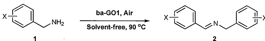
Scheme 1. Oxidation of benzylamine using ba-GO3
