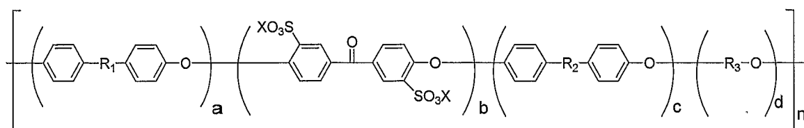
Formula VI
