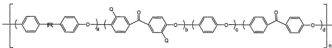
Formula I
