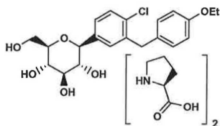
Compound Ih ;
