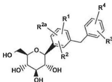
Compound D
