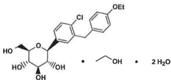
Compound Ic
