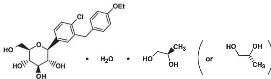
Compound Ib
