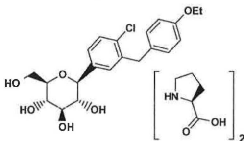
Compound Ih
