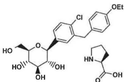
Compound II
