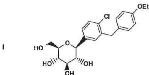
Compound I
