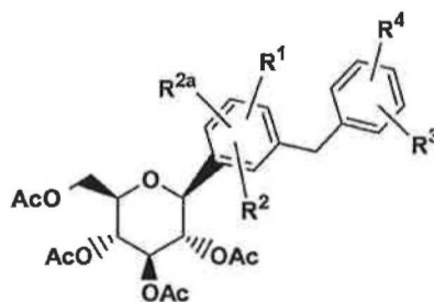
Compound C
