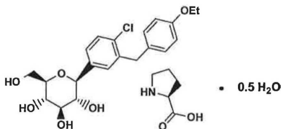
Compound Ij
