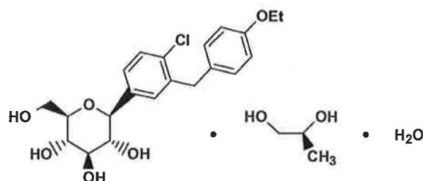
Crystalline (S)-PG (SC-3)
