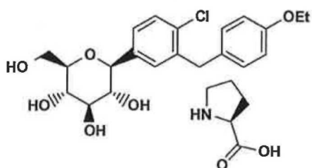
Compound Ii ;
