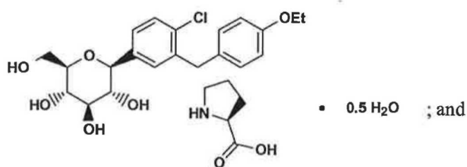
Compound Ij
