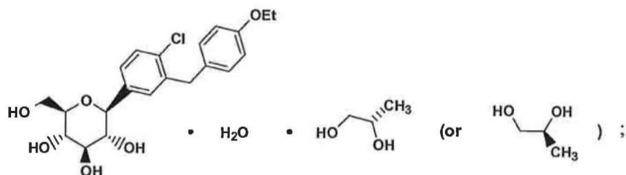
Compound Ia
