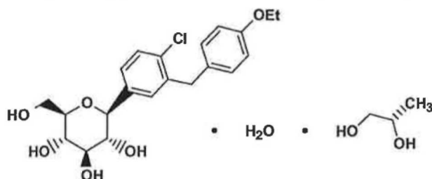
Compound Ia
