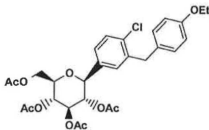
Compound A
