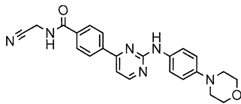
(Compound E).
