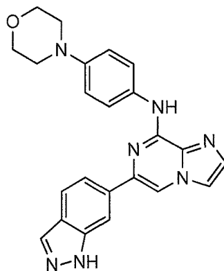
(Compound D).
