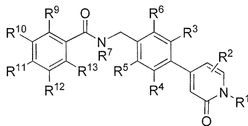
Formula (Ia)
