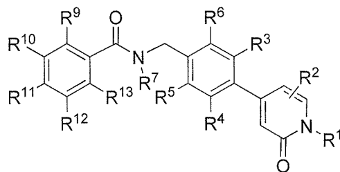
Formula (Ib)
