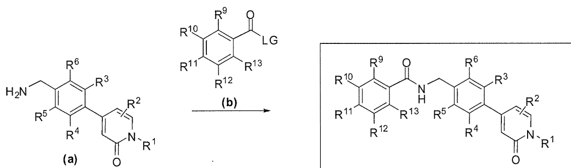
Scheme I
