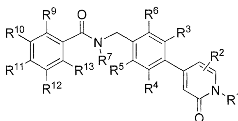
Formula (Ib)
