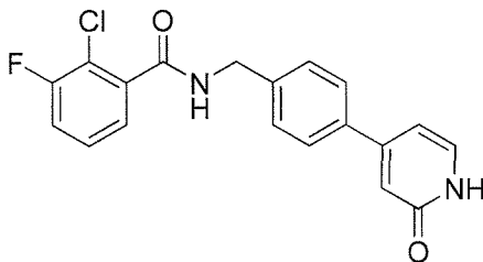
Scheme IX
