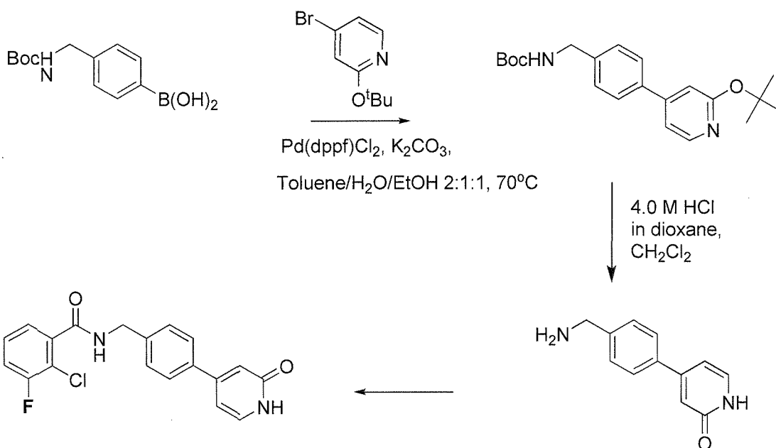
Scheme IX
