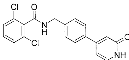
Scheme VIII
