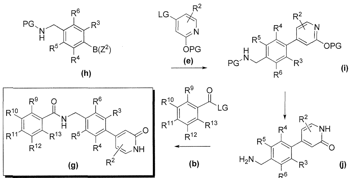
Scheme III
