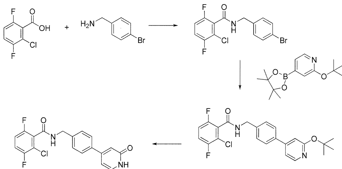
Scheme X
