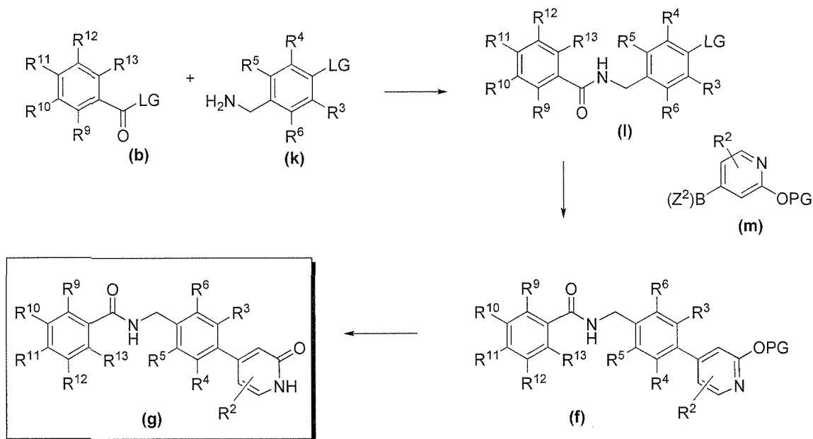
Scheme IV
