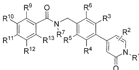
Formula (I)
