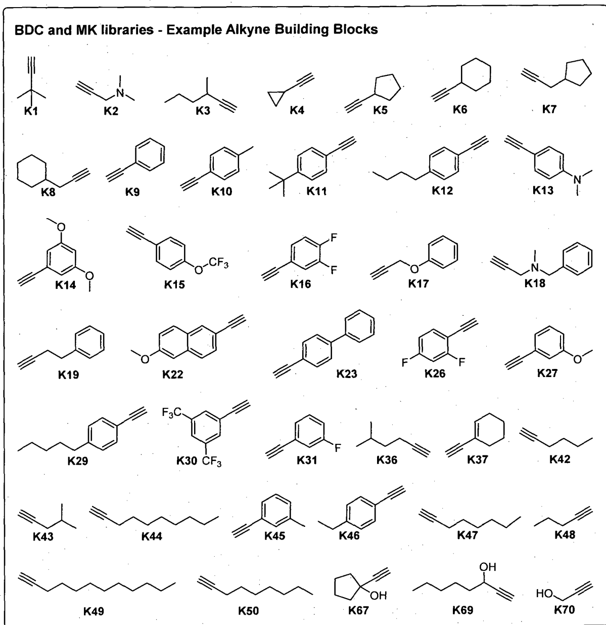
Scheme 4. Alkyne building blocks for the BDC and MK libraries.
