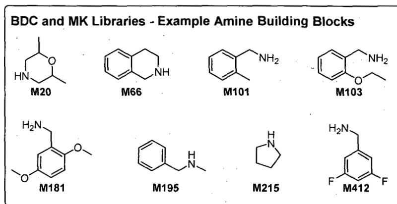
Scheme 3. Amine Building blocks for the BDC and MK libraries.
