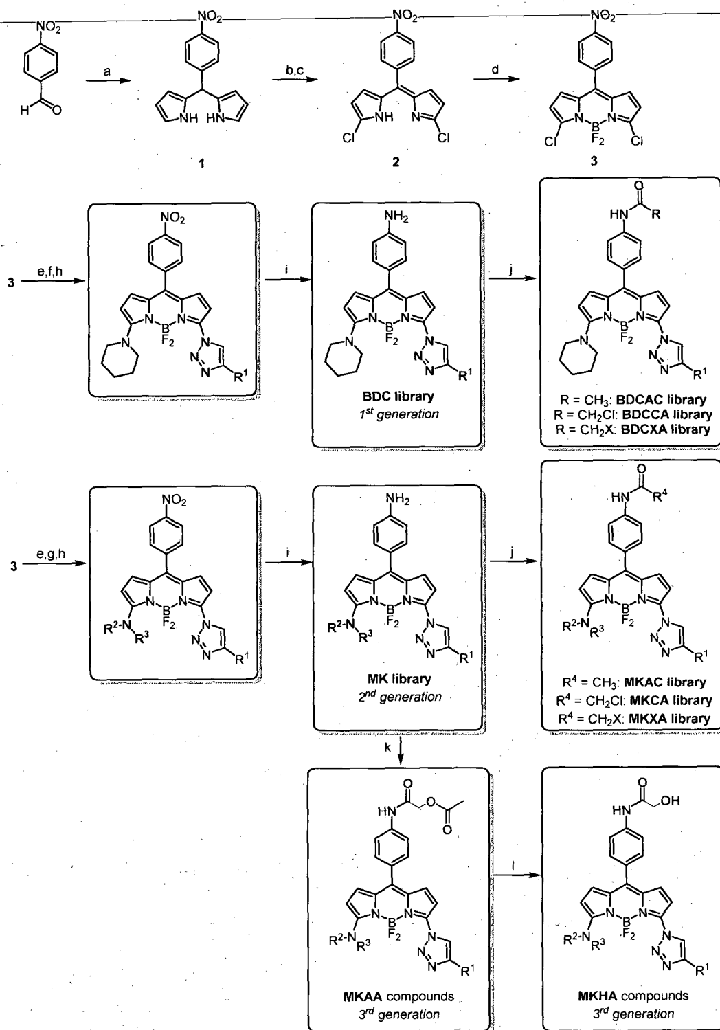
Scheme 2. Solution Phase Synthesis of Amino-Triazolyl BODIPY Compounds.
