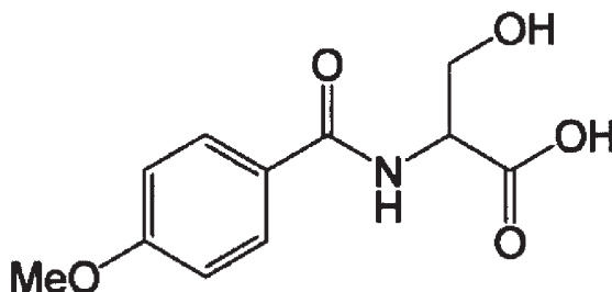
N-(p-methoxybenzoyl)-L-serine (Compound 5)
