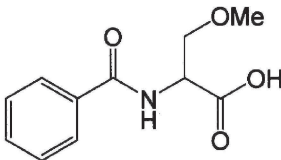
N-benzoyl-DL-O-methylserine (Compound 16)
