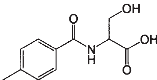
N-(p-methylbenzoyl)-D-serine (Compound 15)
