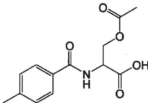
N-(p-methylbenzoyl)-O-acetyl-L-serine (Compound 11)
