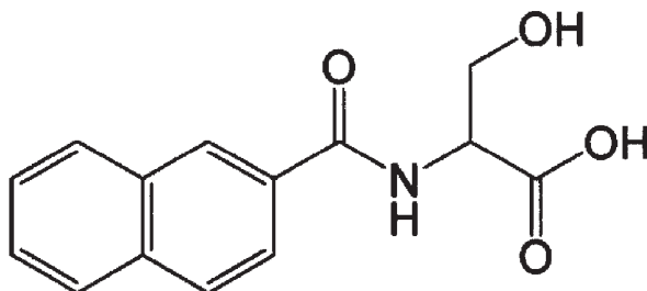
N-(2-naphthoyl)-L-serine (Compound 10)
