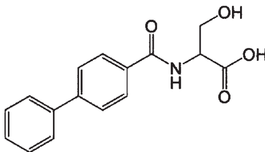
N-(p-phenylbenzoyl)-L-serine (Compound 14)
