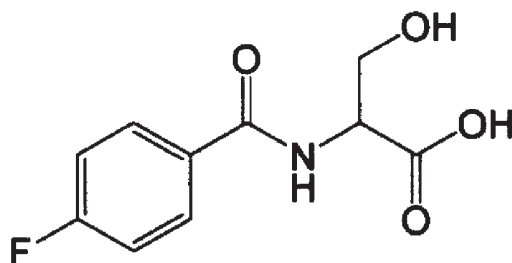
N-(p-fluorobenzoyl)-L-serine (Compound 4)
