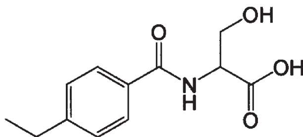
N-(p-ethylbenzoyl)-L-serine (Compound 7)
