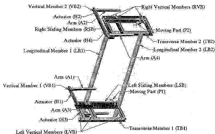
Figure 2: Schematic diagram of a system for folding/unfolding a transport container.
