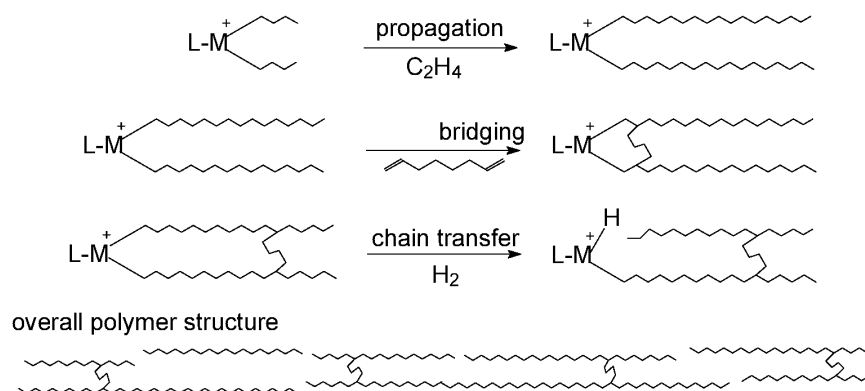
Scheme 4: Illustration of “Ladder Branching” kinetics including the resulting molecular architecture. The metal–ligand catalyst are represented together by L-M^+ .
