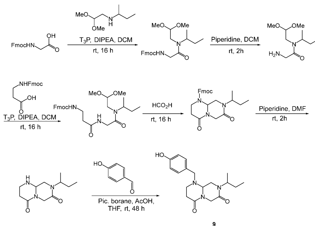
Scheme 10.
