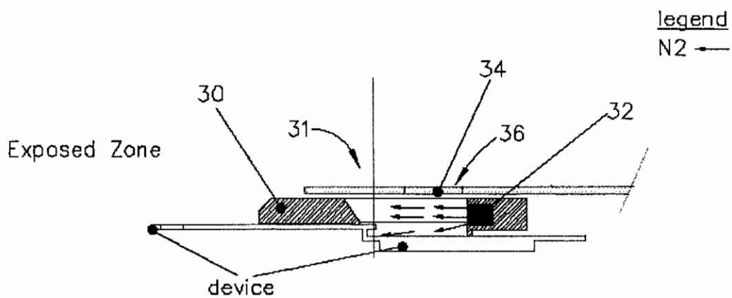
Figure 5 – Bonding area
