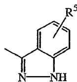
(b-7)
