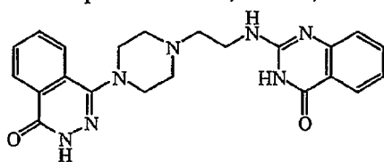
Compound 35
