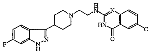
Compound 36
