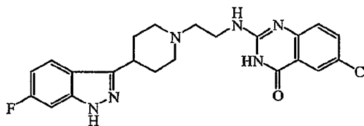
Compound 36
