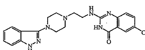
Compound 1
