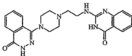
Compound 35
