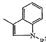
(b-8)
