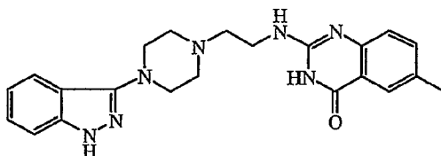
Compound 43
