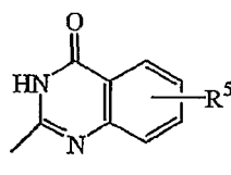
(b-3)
