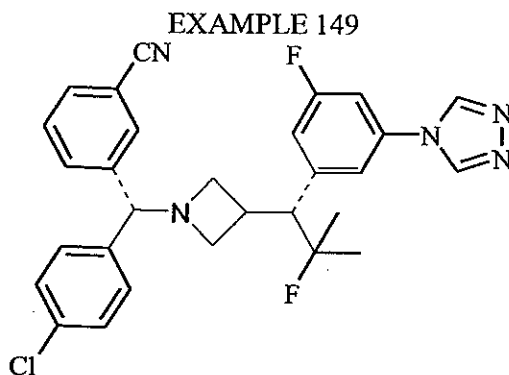
3-[( R )-(4-chlorophenyl)(3-((1 R )-2-fluoro-1-[3-fluoro-5-(4 H -1,2,4-triazol-4-yl)phenyl]-2-methylpropyl)azetidin-1-yl)methyl]benzonitrile
