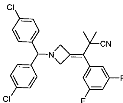
3-{1-[Bis(4-chlorophenyl)methyl]azetidin-3-ylidene}-3-(3,5-difluorophenyl)-2,2-dimethylpropanenitrile
