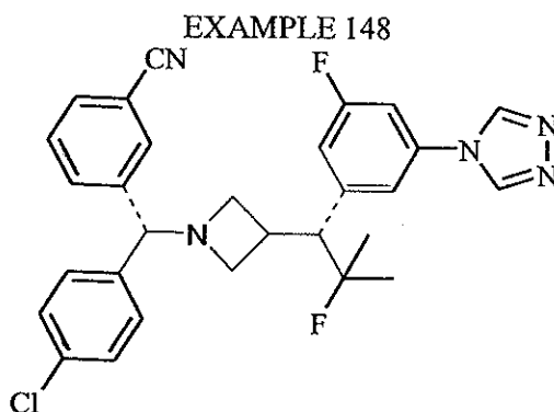
3-[( SR )-(4-chlorophenyl)(3-((1 RS )-2-fluoro-1-[3-fluoro-5-(4 H -1,2,4-triazol-4-yl)phenyl]-2-methylpropyl)azetidin-1-yl)methyl]benzonitrile
