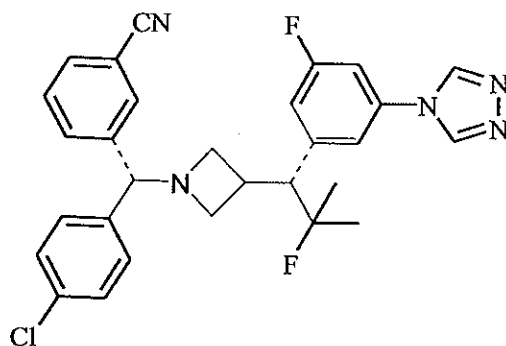
3-[( R )-(4-chlorophenyl)(3-((1 R )-2-fluoro-1-[3-fluoro-5-(4 H -1,2,4-triazol-4-yl)phenyl]-2-methylpropyl)azetidin-1-yl)methyl]benzonitrile
