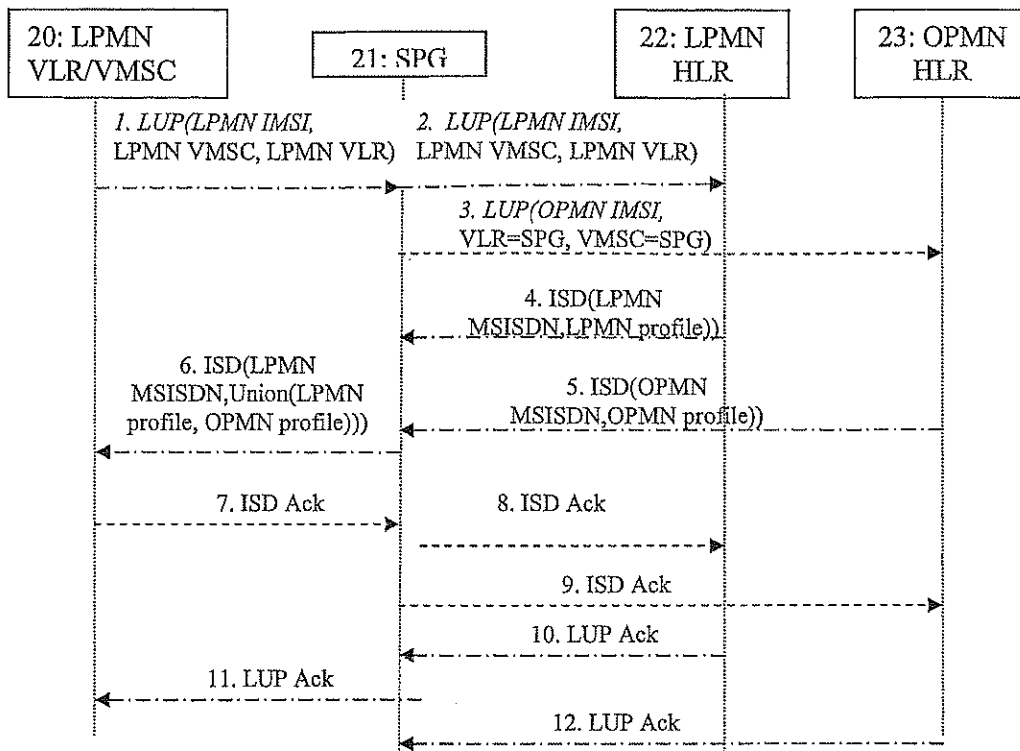
Figure 2 GSM location update and supplementary service profile
