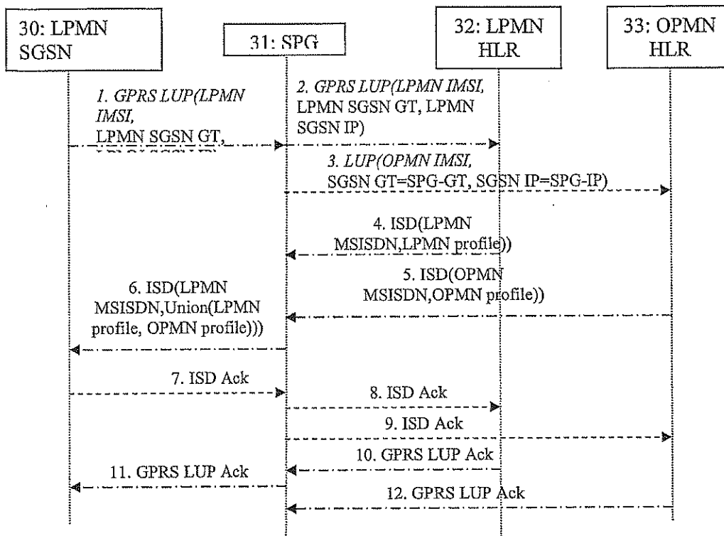
Figure 3: GPRS location update
