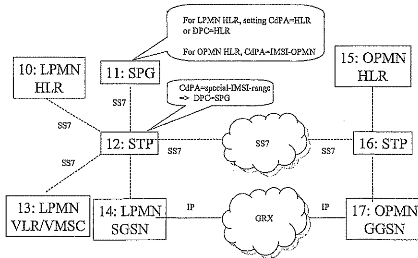
Figure 1: Signal Packet Gateway Network Architecture
