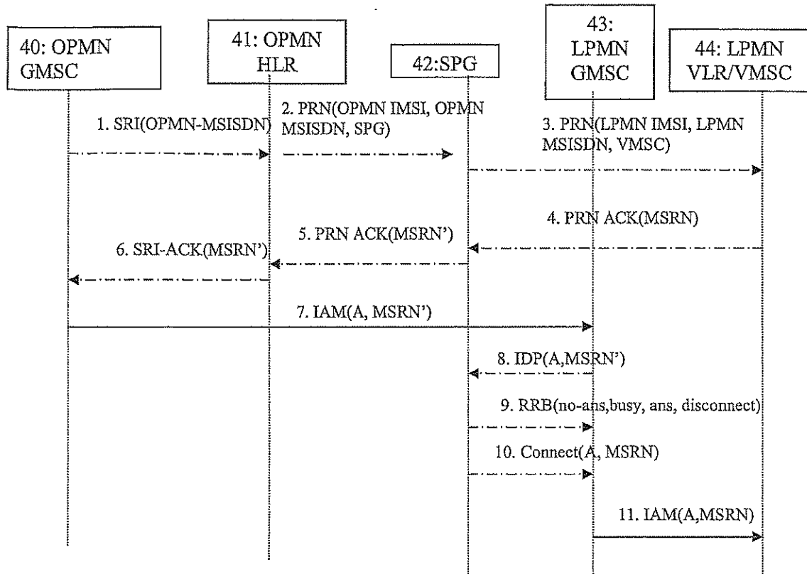
Figure 4: To overseas number
