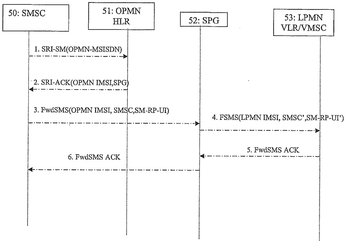
Figure 5: MT SMS To overseas number
