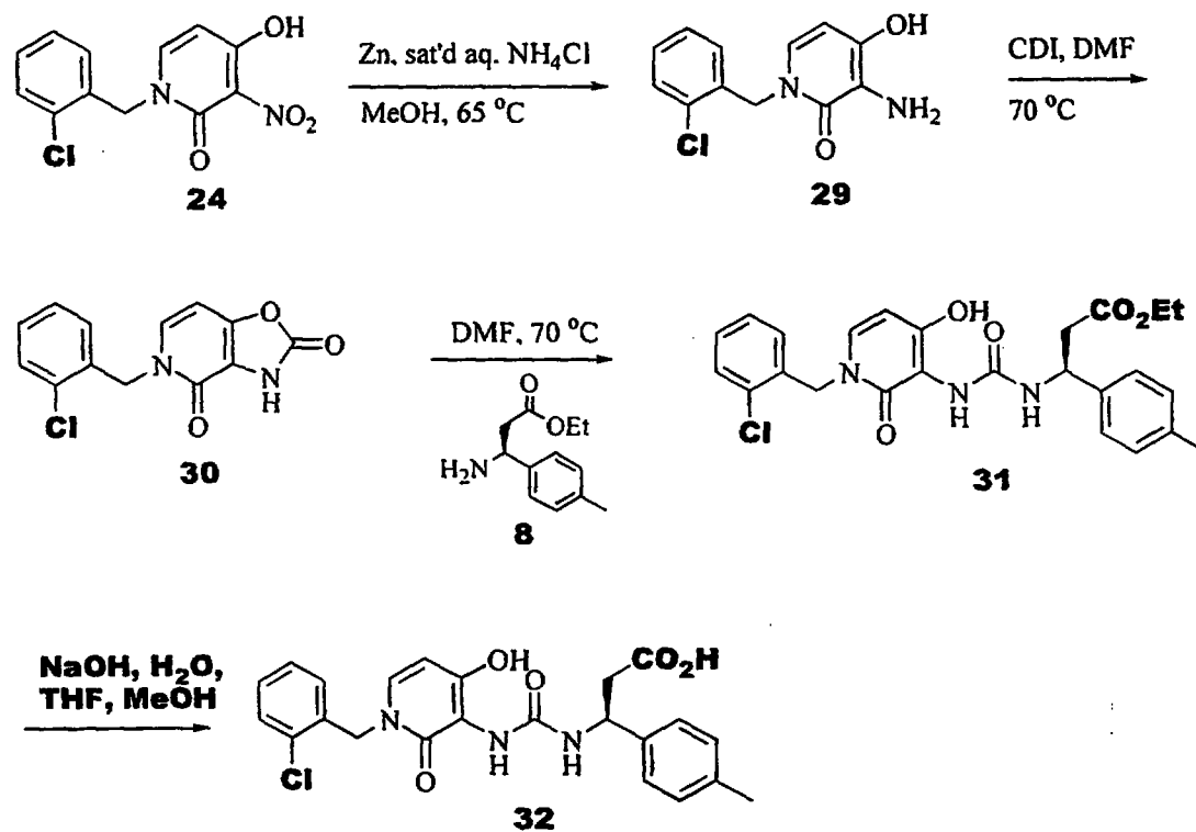
Scheme 8
