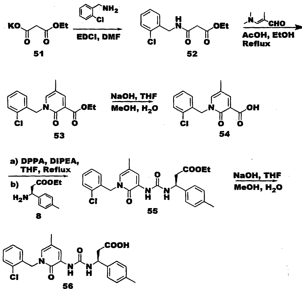
Scheme 14
