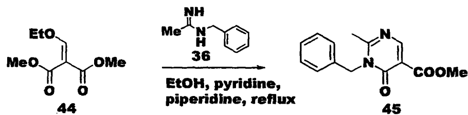
Scheme 11
