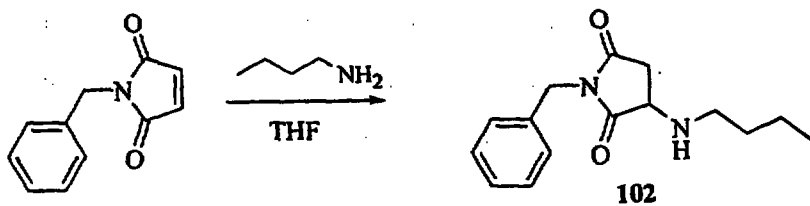
Scheme 19
