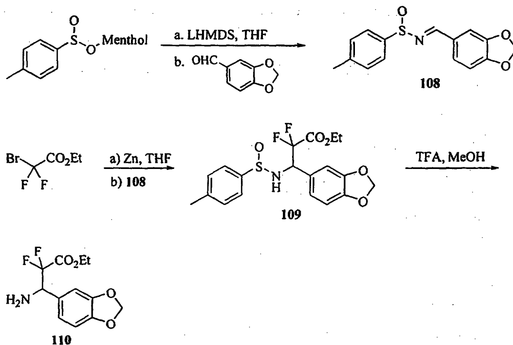
Scheme 22
