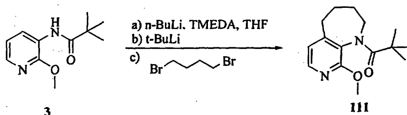
Scheme 23
