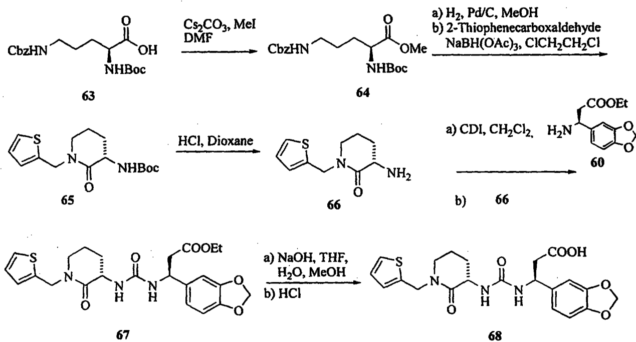
Scheme 16
