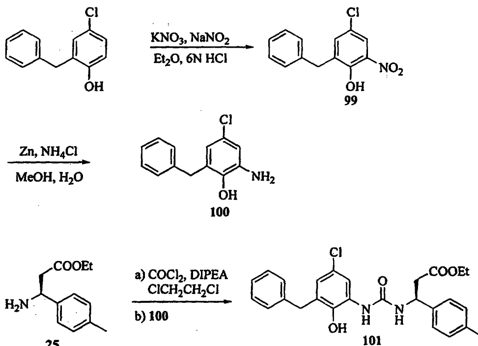
Scheme 18
