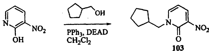
Scheme 20
