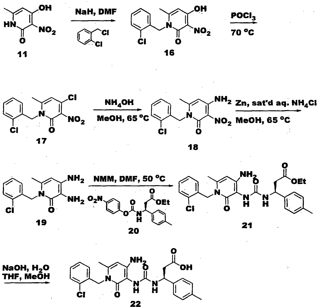
Scheme 3
