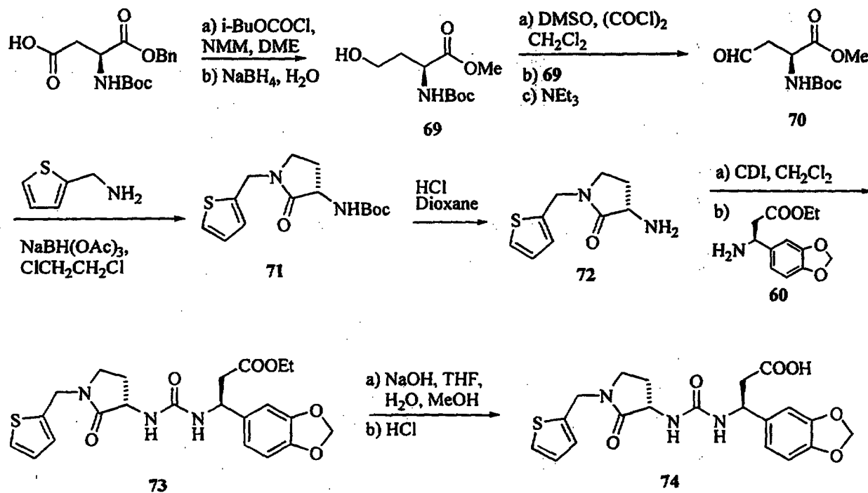
Scheme 17
