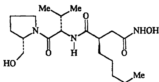
Actinonin
